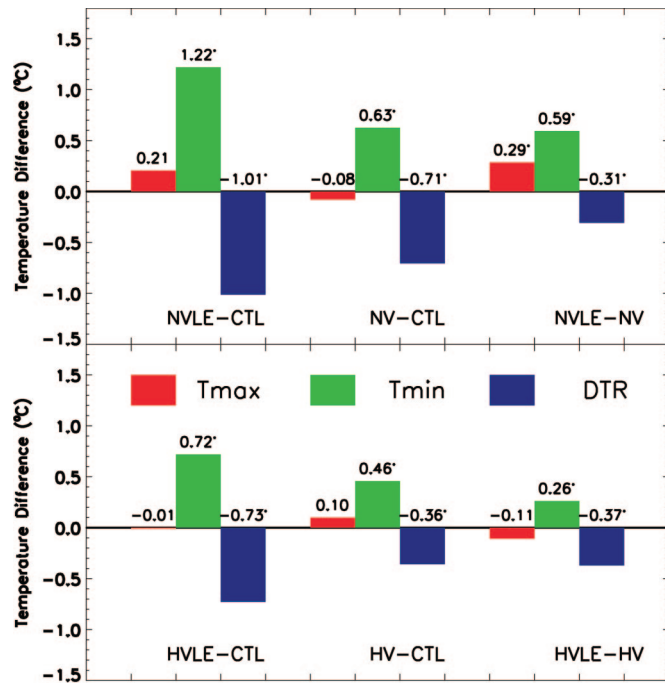
Fig. 5. Simulated annual mean T_{\max} , T_{\min} , and DTR differences ( ^{\circ}\text{C} ) among the four experiments (NVLE, NV, HVLE, and HV) and the control run (CTL) under clear-sky conditions averaged over the Sahel. The clear-sky conditions are defined as in Fig. 3. The temperature differences marked with * are statistically significant at the 5% level. The significance test was done as for Fig. 3.
