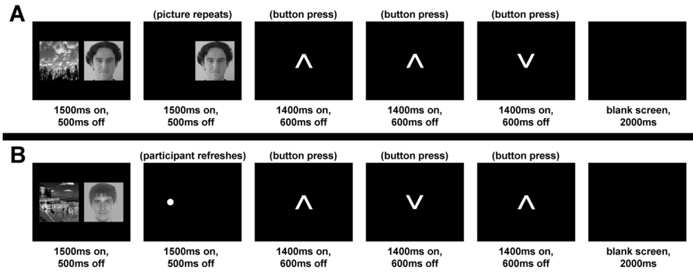
Figure 1. Task designs
