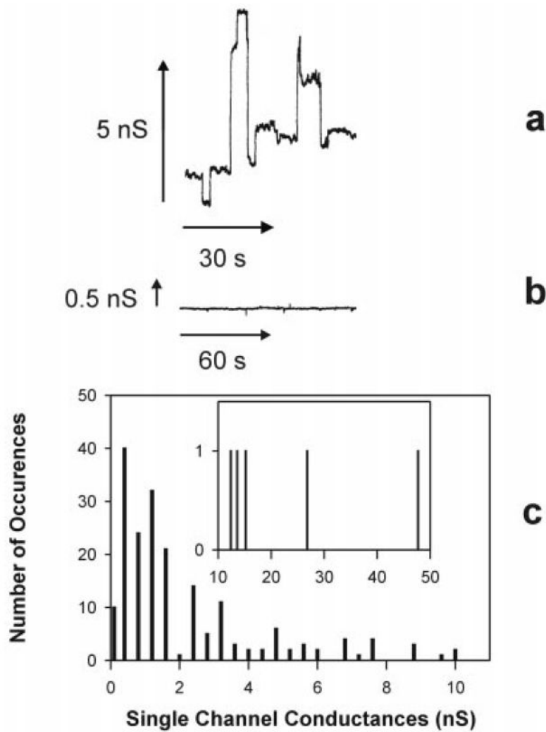
Fig. 5. C 16 -Ceramide forms channels in planar phospholipid membranes
