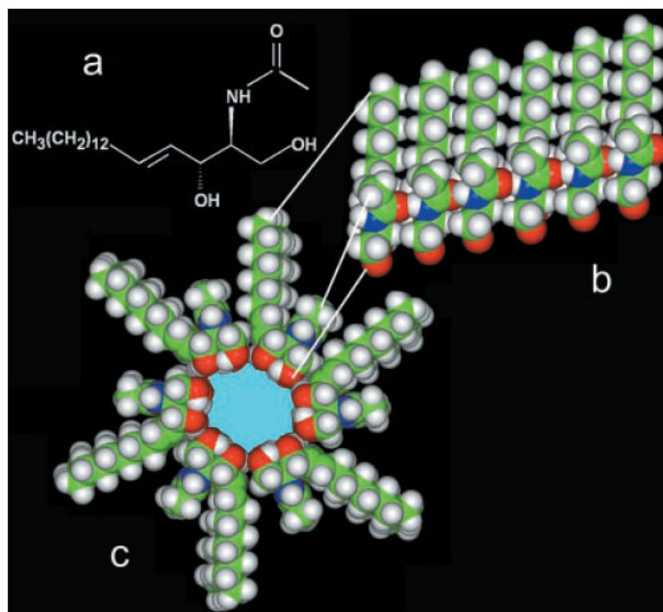
Fig. 3. Structural model for ceramide pore formation
