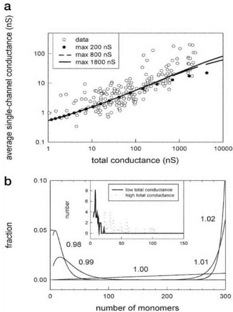
Fig. 4. The average size of ceramide channels increased with increasing ceramide content in the membrane
