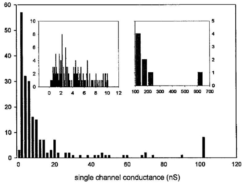
Fig. 2. Distribution of single channel conductances produced by 5 \mu\text{M} \text{C}_2 -ceramide Data were compiled from four separate experiments using the conditions stated for Fig. 1, a-c . Only distinct vertical current increments were measured. The left and right insets are detailed distributions of channels with single channel conductances below 10 nS and greater than 100 nS, respectively.
