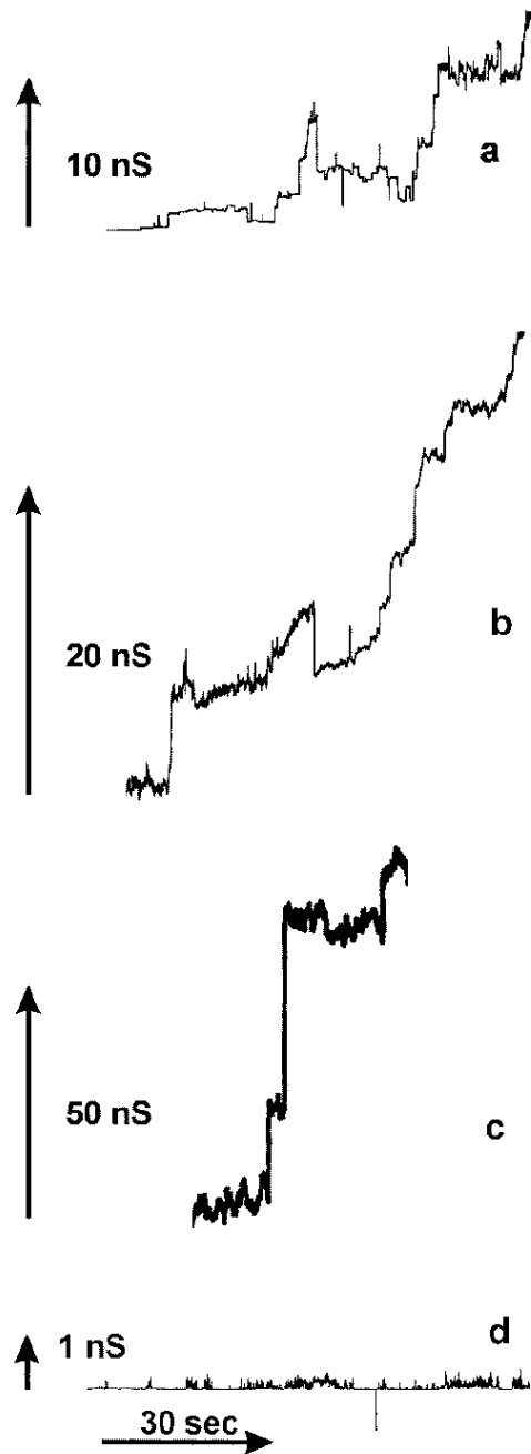
Fig. 1. C 2 -ceramide forms channels in planar phospholipid membranes a–c , continuous current recordings of channel formation induced by the addition of 5 \mu\text{M} C 2 -ceramide to the aqueous solution, which consisted of 1 M KCl, 1 mM MgCl 2 , and 5 mM MES (pH 6). The applied voltage was clamped at 9 mV. d , current recordings in the presence of 120 \mu\text{M} C 2 -dihydroceramide. Conditions were as in a–c .
