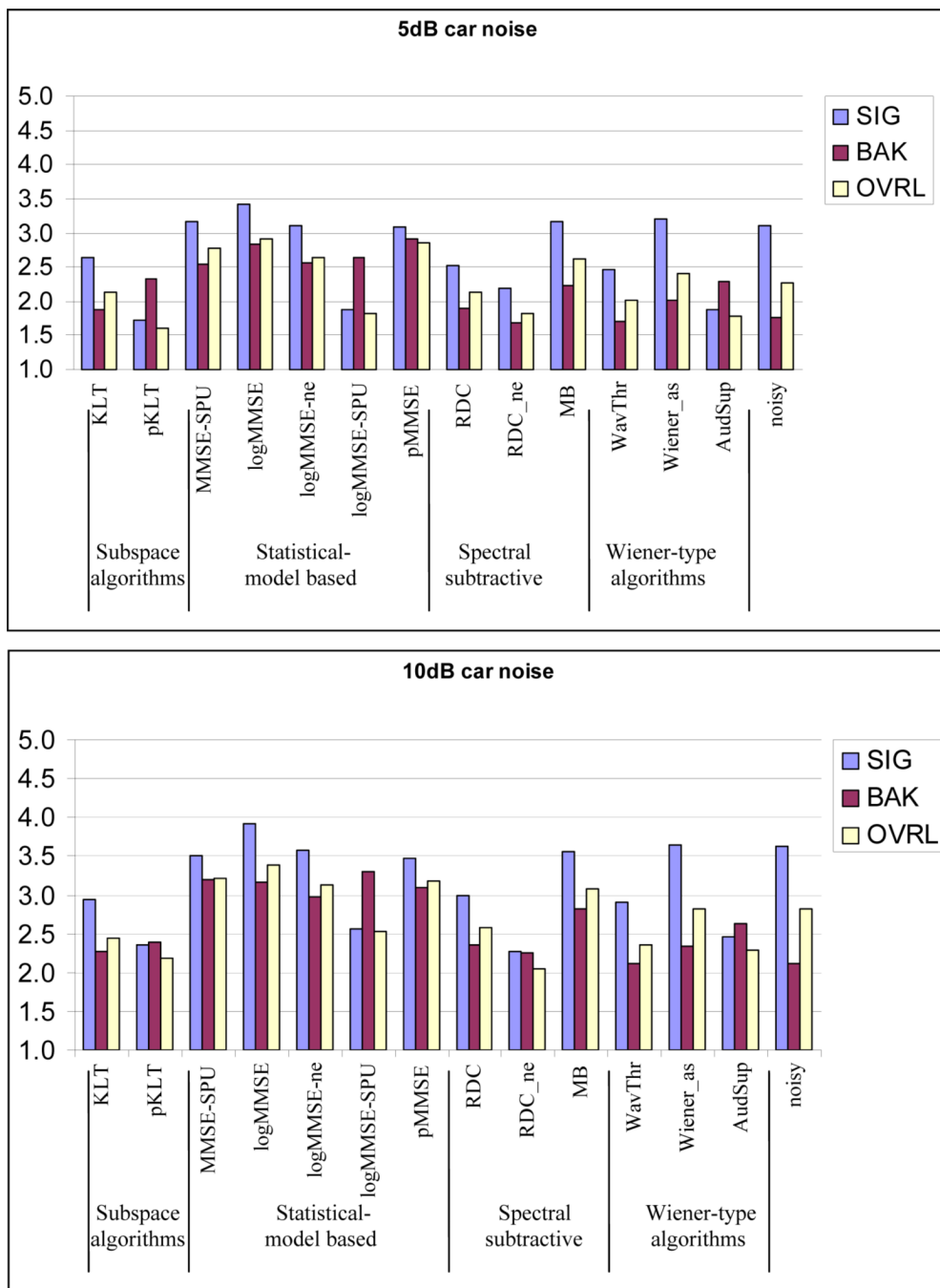
Fig. 4. The mean scores for SIG, BAK, and OVRL scales for the 13 methods evaluated in car noise background and for SNR levels of 5dB and 10dB
