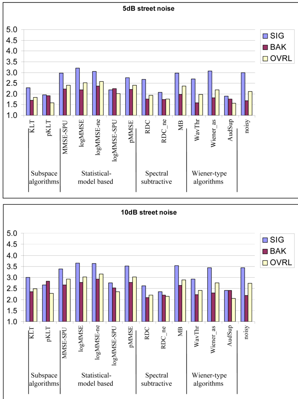
Fig. 5. The mean scores for SIG, BAK, and OVRL scales for the 13 methods evaluated in street noise background and for SNR levels of 5dB and 10dB
