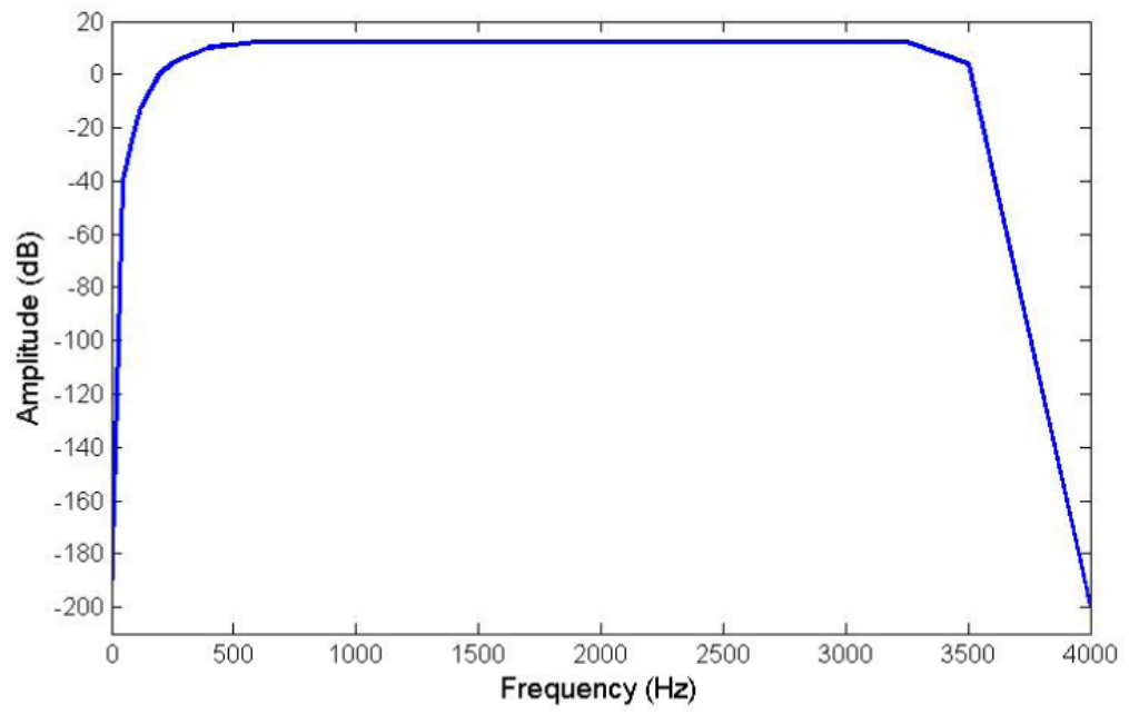
Fig. 2. Frequency response of IRS filter.
