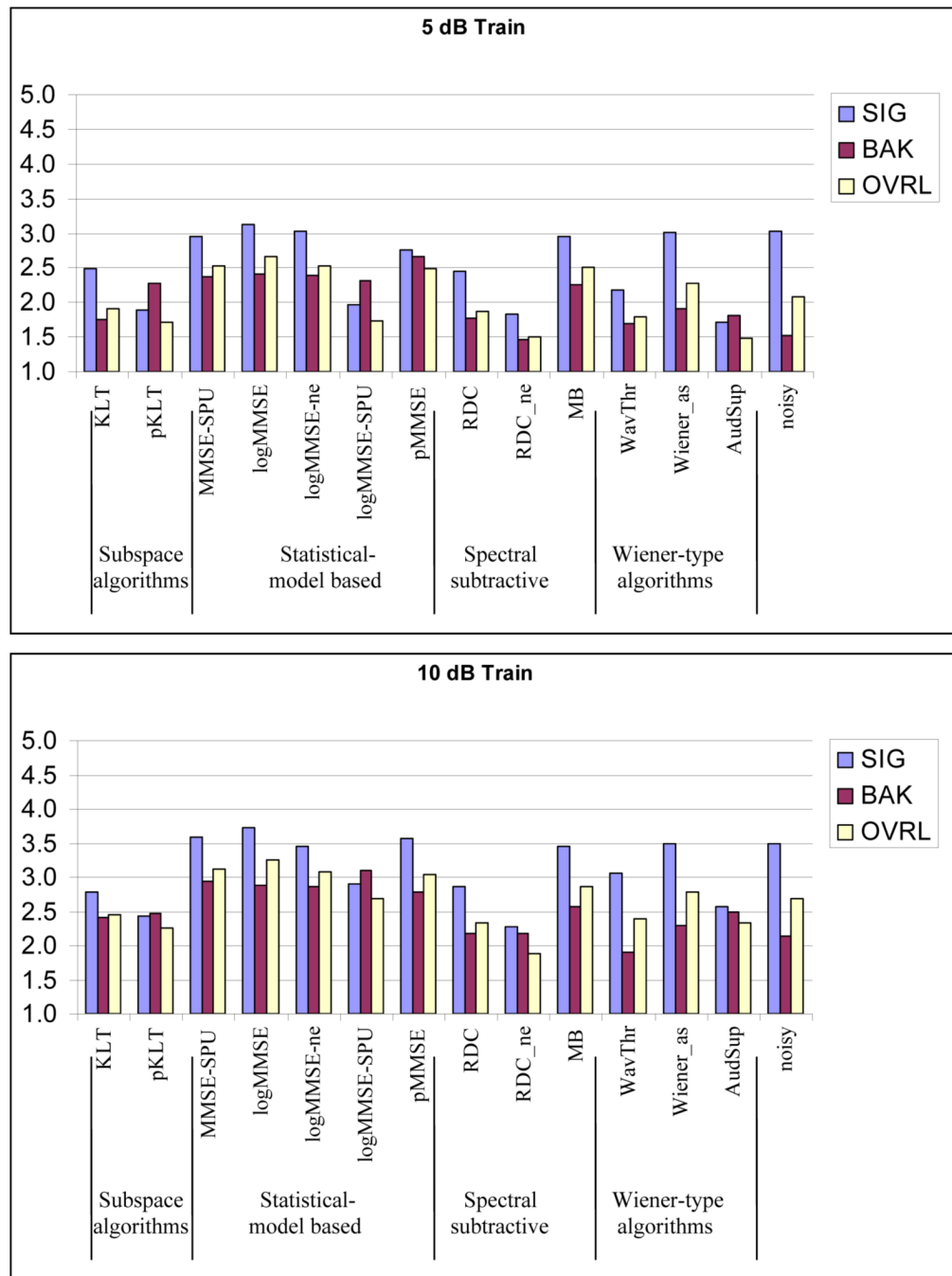
Fig. 6. The mean scores for SIG, BAK, and OVRL scales for the 13 methods evaluated in train noise background and for SNR levels of 5dB and 10dB
