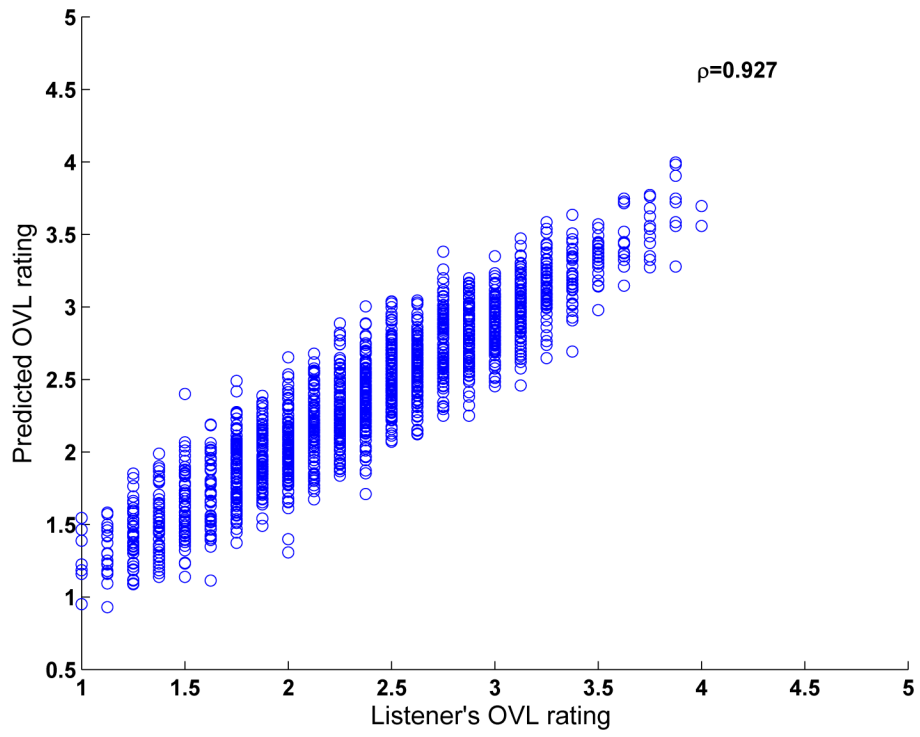
Fig. 7. Regression analysis of listener's OVL ratings, based on SIG and BAK ratings.
