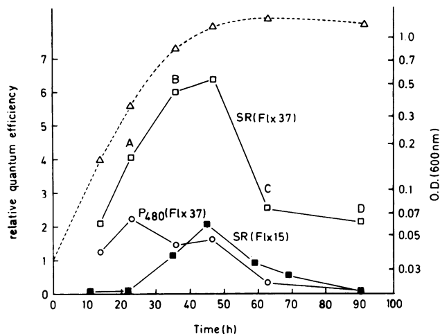
FIG. 1. Time course for the activities of P_{480} and SR during growth of H. halobium Flx37 and Flx15. Receptor activities were determined as described in Materials and Methods, and growth followed by turbidity changes was measured at 600 nm ( \Delta , log scale). Times at which receptor concentrations were determined (A to D) by difference spectroscopy on isolated cell membranes are indicated (see Fig. 2).
