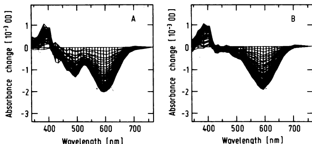
FIG. 4. Difference spectra of cell membrane fractions from cells after 24 h of growth before (A) and after (B) being washed with Tween 20 as described previously (13).
