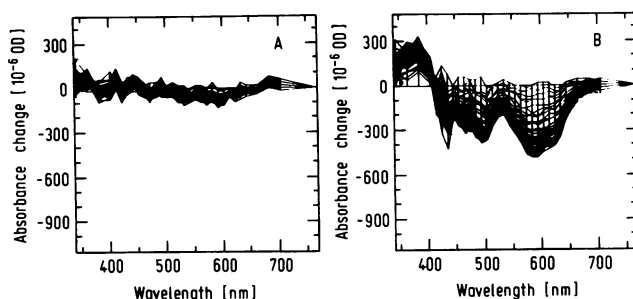
FIG. 5. Reconstitution of P 480 and SR. Difference spectra of membrane fractions from cells grown in the presence of 2 mM nicotine for 24 h before (A) and after (B) incubation with all- trans retinal.
