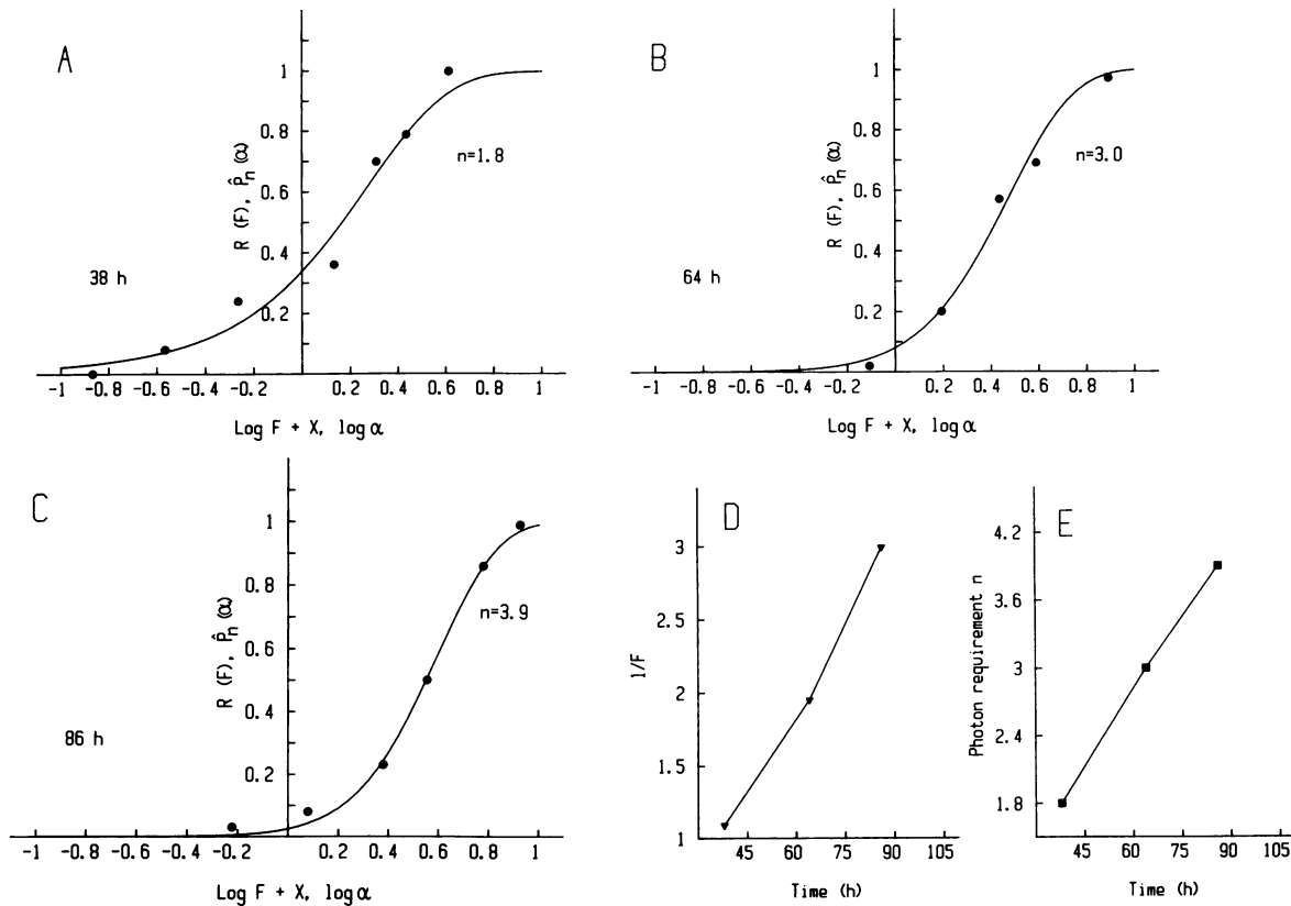
FIG. 7. Photon requirement of the SR-dependent photophobic response in halobacteria at various stages of growth. (A to C) Cells of strain Flx37, grown in a 100-ml Erlenmeyer flask, were exposed to constant orange background light ( 72 \text{ W/m}^2 ) and were stimulated with flashes of near-UV light (366 nm). For each datum point, 60 to 90 cells were used and the averaged result was fitted to theoretical Poisson distribution curves by the least-square method. (For details see references 3 and 6). The x value is different in each plot. (D) The inverse value of the photon exposure ( F ) necessary for absorption of one efficient photon as a function of cell growth. The value 1/F is proportional to the number of active photoreceptor molecules in the cell. A value of 1 for F equals 1.4 \cdot 10^{-5} \text{ mol/m}^2 . (E) Minimal number of photons necessary to elicit a photophobic response as a function of cell growth. The data for panels D and E are derived from those in panels A to C. Note that the time scale in this figure may be shifted compared with that in Fig. 1 and 3, since kinetics of the cell growth in a fermenter is different from that of a shaker culture.
