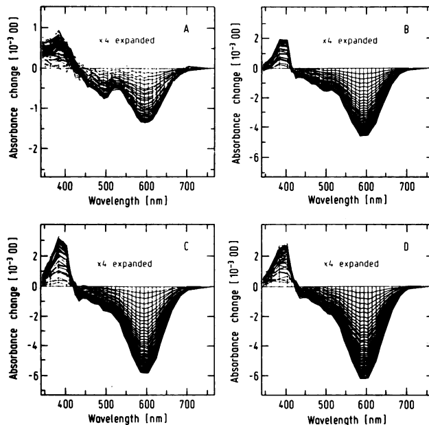
FIG. 2. Difference spectra of membrane fractions from Flx37 cells after 23 (A), 36 (B), 63 (C), and 91 (D) h of growth. The spectra were recorded at room temperature in 10-ms time intervals between 0 and 500 ms after the white light used simultaneously for actinic action and for monitoring absorbance changes was turned on. Cell membrane fractions were suspended in 4 M NaCl, and sample concentrations were 1.5 optical density units at 400 nm.
