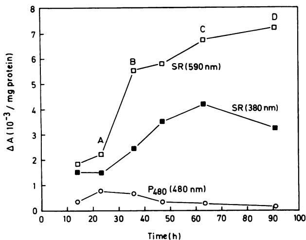
FIG. 3. Absorbance changes of membranes normalized to 1 mg of total membrane protein from cells of different ages grown in a 10-liter fermenter. The apparent decrease of P 480 might be artificial, due to difficult evaluation of the complex spectra in Fig. 2. Times at which absorbances were determined (A to D) are indicated.
