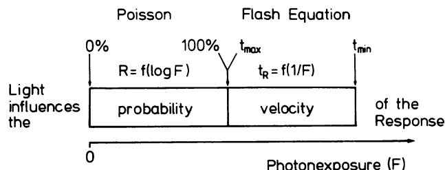
FIG. 6. Scheme for the application of stimulus-response curves to the photophobic response in H. halobium covering the stochastic and kinetic range as described in the text.
