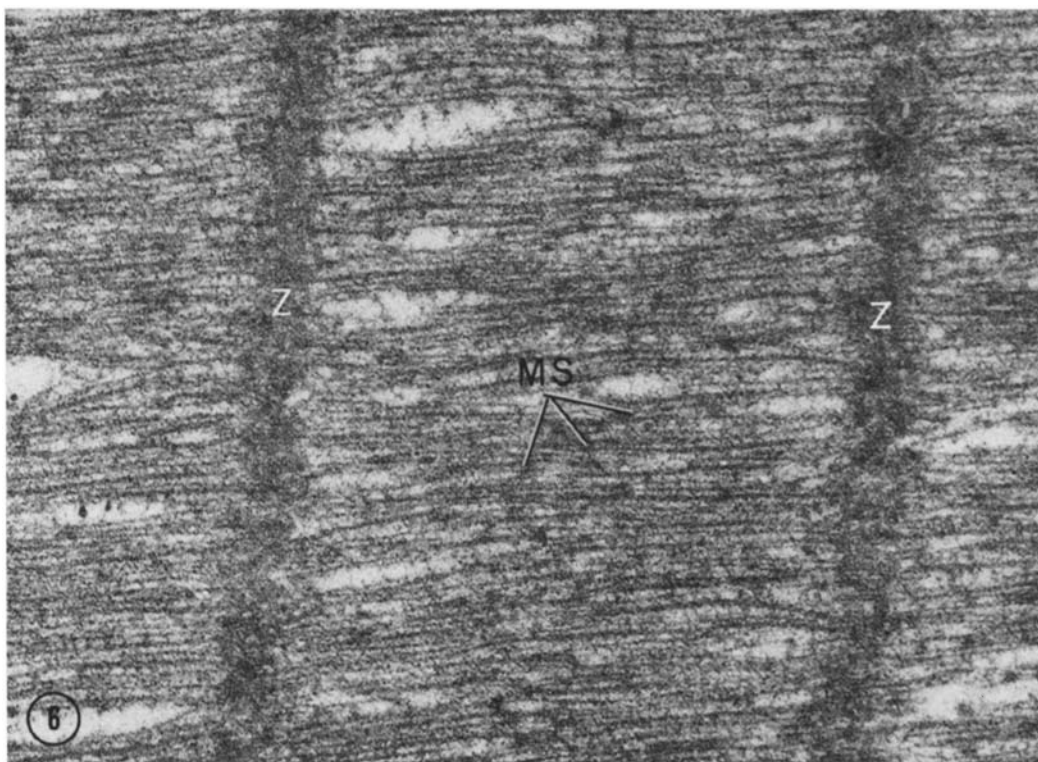
FIGURE 6 Structural disruption of this sample removed from muscle after 24 hr storage at 37°C is apparent. M line segments ( MS ) are displaced both to the left and to the right of the normal M line location. Absence of I bands and thickening of the area around the Z line indicates that supercontraction has occurred. Section stained with uranyl acetate and lead citrate. \times 59,500 .
