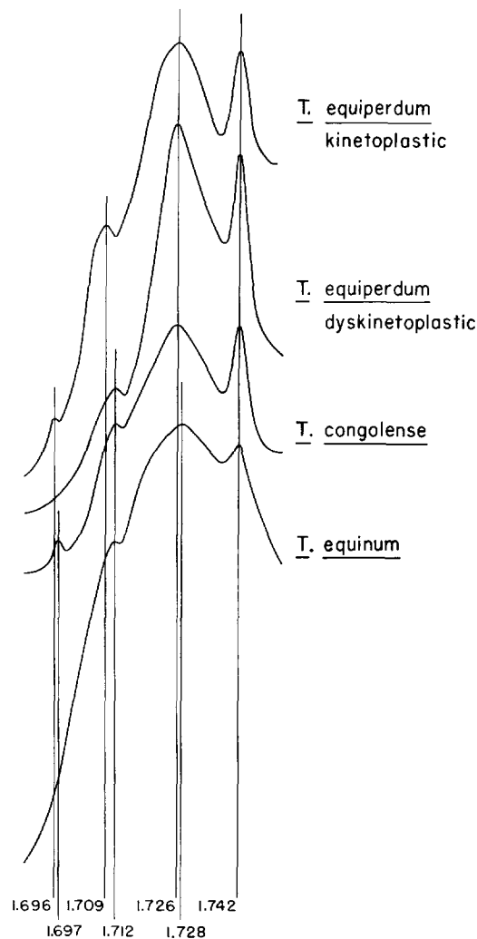
FIGURE 14 Microdensitometer tracings of ultraviolet photographs of cesium chloride buoyant density gradients of DNA from whole cells of the four strains of trypanosomes indicated. In each case the DNA was heated at 100°C for 5 min and then quenched in ice. The reference band (1.742) to the right is native DNA of SPO1.
