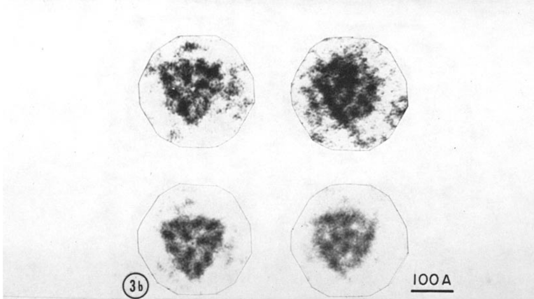
FIGURE 3 Cross-section of the myosin filaments of glycerinated muscle taken in the pseudo-H-zone (region in the middle of the A band where no myosin cross-bridges are present) but not including the M band. Fig. 3 a, area from which the filaments shown in Fig. 3 b were taken. Fig. 3 b, The top two images are of different filaments enlarged from the micrograph in Fig. 3 a. The rotated images below were rotated in 120^\circ intervals.
