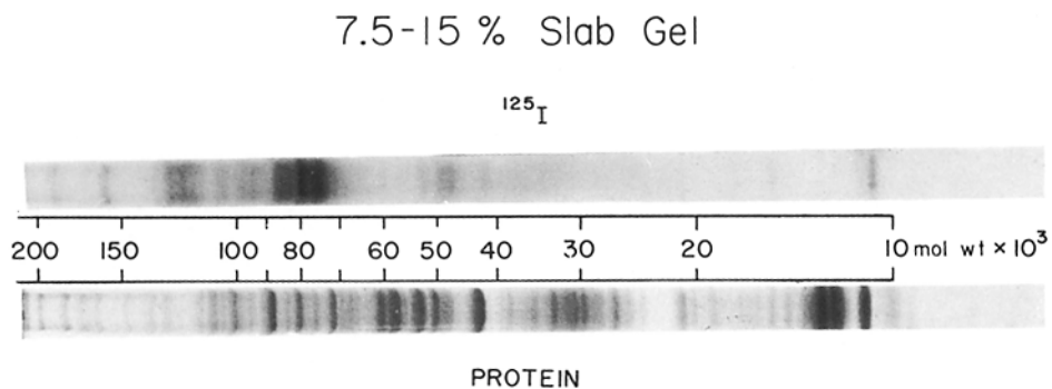
FIGURE 7 SDS polyacrylamide tube and slab gel electrophoresis patterns of iodinated L cells. Top gels ( I ): 7.5% acrylamide, 35:1 A/MBA, 6 mm diameter, 10-cm long tubes; electrophoresis 15 h at 6 mA/gel; gels stained with Coomassie blue, cut, and 1.8 mm sections counted. Middle gels ( II ): 7.5% acrylamide, 35:1 A/MBA (resolving gel), 3.0% acrylamide, 35:1 A/MBA (spacer gel), 1-mm thick, 13-cm long slab, electrophoresis 7 h at 10 mA; gels stained with Coomassie blue (protein), dehydrated, and exposed 15 days to X-ray film ( ^{125}\text{I} ). Bottom gels ( III ): 7.5% to 15.0% continuous gradient acrylamide, 35:1 A/MBA (resolving gel), 3.0% acrylamide, 35:1 A/MBA (spacer gel) 1 mm thick, 20-cm long slab, electrophoresis 20 h at 5 mA; gels stained with Coomassie blue (protein), dehydrated, and exposed to X-ray film for 3 days ( ^{125}\text{I} ).
