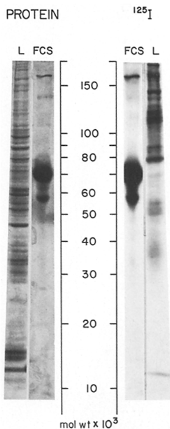
FIGURE 8 SDS polyacrylamide gradient slab gel electrophoresis patterns of iodinated FCS and iodinated intact L cells. Gels were stained for protein with Coomassie blue (left), dehydrated, and exposed to X-ray film for 17 days (FCS) or 30 days (L cells) (right). Resolving gel composition 7.0%–13% acrylamide, 35:1 A/MBA, 1 mm thick, 20 cm long. Electrophoresis 15 h at 7.5 mA.
