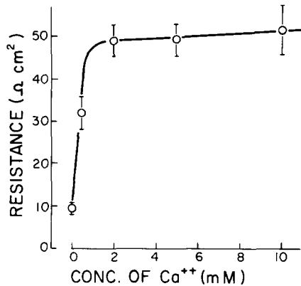
FIGURE 8 Recovery of the electrical resistance as a function of the concentration of Ca 2+ of the bathing solution. Once the junctions were opened with Ca-free MEM and EGTA, the disks were divided into several groups. To recover, each disk was placed in MEM with different concentrations of Ca 2+ . The electrical resistance was measured at 90 min, i.e., before the recovery was completed.
