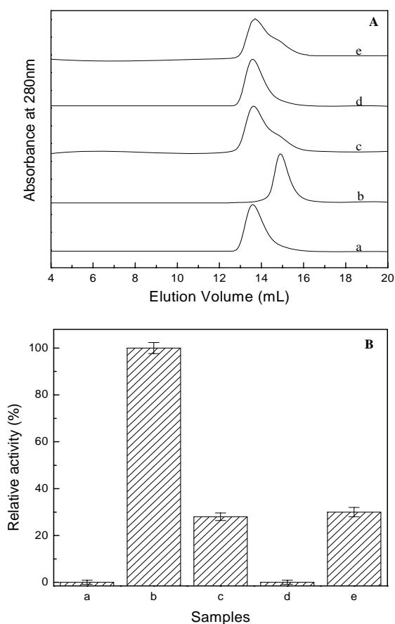
Figure 4 Deciphering the reversibility of the tetramer-dimer transition. A. SEC profile of PfGST . Curves a-e represent tetrameric PfGST , dimeric PfGST , dimeric PfGST dialyzed for 4 h in buffer devoid of GSH, dimeric PfGST dialyzed for 24 h in buffer devoid of GSH, dimeric PfGST loaded on the column equilibrated and run with buffer without GSH. The curves have been displaced on Y-axis for presentation. B. Enzymatic activity assay of the eluted peaks. In the figure, bars a-e represents data for the peaks described in 4A.
