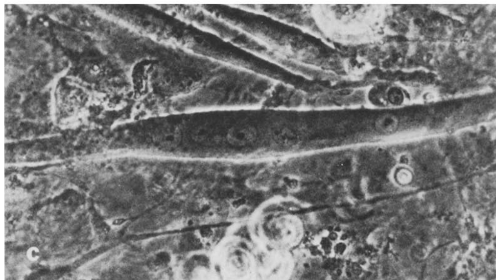
FIGURE 2 Rat myotube in primary culture, labeled with R-Bgt. (a) TIRF. \theta = 72.5^\circ ; d = 120 nm. Note that only the large AChR patch in the middle of the field and a small one near the top become visible. (b) Epifluorescence of the same field. (c) Phase contrast of the same field. A \times 40 phase-contrast water-immersion objective with a numerical aperture of 0.75 and a free working distance of 1.4 mm was used. Bar, 30 \mu\text{m} .
