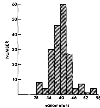
FIGURE 11 A histogram of lengths of 95K protein after rotary shadowing as in Fig. 9 a.
