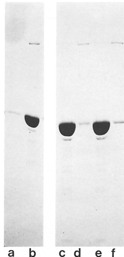
FIGURE 6 Sedimentation of 95K and F-actin. Actin at 9.5 \mu\text{M} and 95K at 0.24 \mu\text{M} were incubated for 30 min at 25^\circ\text{C} in the buffer in Fig. 3 at pH 6.8 or 7.8 and sufficient \text{CaCl}_2 to achieve free \text{Ca}^{++} concentrations of 0.1 or 10 \mu\text{M} . F-actin was pelleted at 100,000 \text{ g} for 30 min in a Beckman airfuge (Beckman Instruments, Inc., Spinco Div., Palo Alto, CA) at 25^\circ\text{C} . (a, b) pH 6.8, 0.1 \mu\text{M Ca}^{++} , (a) pellet, (b) supernatant. (c, d) pH 6.8, 10 \mu\text{M Ca}^{++} , (c) pellet, (d) supernatant. (e, f) pH 7.8, 0.1 \mu\text{M Ca}^{++} , (e) pellet, (f) supernatant.
