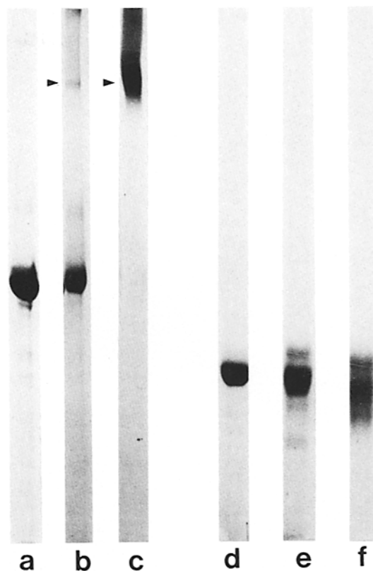
FIGURE 2 SDS PAGE of dimethyl suberimide (DMSI) cross-linking of 95K. Conditions were 0.2 mg/ml protein in 0.2 M triethanolamine, pH 8.5, and 1 mg/ml DMSI. Reaction was allowed to proceed for 0 (a, d), 1 (b, e), or 12 h (c, f) at 0^\circ\text{C} . a-c 95K, (d-f) bovine serum albumin (BSA). The 95K is cross-linked to a species measuring 190,000 daltons (arrow) while BSA, a monomeric protein, retains its monomeric molecular weight.
