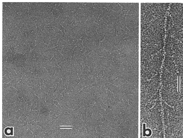
FIGURE 8 Structure of 95K protein after negative staining in uranyl acetate. (a) Field of 95K protein stained from a solution containing 0.5 μM protein in 0.1 μM Ca 2+ . (b) F-actin at 0.15 μM labeled with 0.1 μM 95K protein in 0.1 μM Ca 2+ . Proteins were incubated in the buffer described in Fig. 7. Bars: (a) 80 nm, (b) 40 nm. (a) × 62,500. (b) × 175,000.
