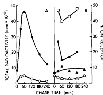
FIGURE 4 Kinetics of oligosaccharide phosphorylation and receptor binding. A shows the total radioactivity recovered as phosphorylated oligosaccharides as a function of chase time both in the nonreceptor-bound fraction (●) and the Man 6-P eluate of Thy + cells (○). In B, the percent of each phosphorylated species recovered in the Man 6-P eluate is shown as a function of chase time. The species are: Δ, 1 phosphodiester; ▲, 2 phosphodiester; ■, 1 phosphomonoester; □, 2 phosphomonoester.
