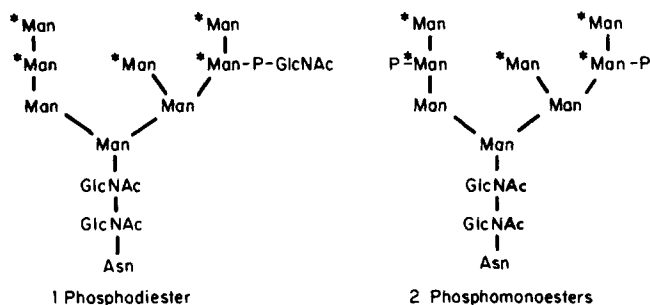
FIGURE 1 Representative structures of high mannose oligosaccharides containing phosphodiester and phosphomonoesters. The species shown contain eight mannose residues but the actual number may vary from six to nine; the asterisks indicate the mannose residues which may be phosphorylated (9). Oligosaccharides may contain one or two phosphate residues.
