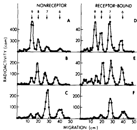
FIGURE 5 Size of the underlying high mannose-type oligosaccharide units derived from nonreceptor-bound (A, B, and C) and receptor-bound (D, E, and F) phosphorylated oligosaccharides. Species containing one phosphodiester, obtained after 60 (A and D) and 240 (B and E) min of chase, and one phosphomonoester, obtained after 120 min of chase (C and F) were neutralized and fractionated by paper chromatography. The migration position of standard high mannose-type oligosaccharides containing \text{Man}_9\text{GlcNAc} (9), \text{Man}_8\text{GlcNAc} (8), \text{Man}_7\text{GlcNAc} (7), and \text{Man}_6\text{GlcNAc} (6) are indicated in A and D.
