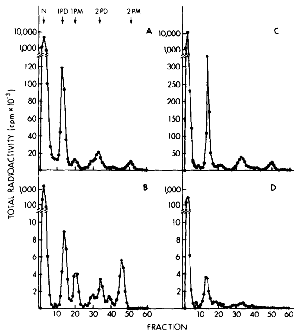
FIGURE 2 QAE-Sephadex fractionation of phosphorylated oligosaccharides. The endo H digests of the nonreceptor-bound 3 H-labeled glycopeptides (A and C) and those obtained from the Man 6-P eluates (B and D) were applied to QAE-Sephadex columns (5 ml) equilibrated in 2 mM pyridinium acetate, pH 5.3. The columns were eluted with linear pyridinium acetate gradients (200 ml) from 2 to 500 mM, and 2-ml fractions were collected; no radioactive species eluted beyond fraction 60, so that abbreviated profiles are shown. The elution positions of neutral oligosaccharides (N) as well as oligosaccharides with one phosphodiester (1PD), one phosphomonoester (1PM), two phosphodiesters (2PD), and two phosphomonoesters (2PM) are shown in A. The fractions were obtained from Thy + cells (A and B) and P388D 1 cells (C and D) after a 60-min labeling with [2- 3 H]mannose. The Man 6-P eluate contained 6.3% of the total 3 H-mannose-labeled radioactivity in Thy + cells and 5.3% of the radioactivity in P388D 1 cells. The break in the ordinate represents a shift between two linear scales.
