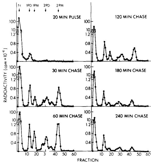
FIGURE 3 QAE-Sephadex fractionation of Man 6-P-eluted phosphorylated oligosaccharides obtained from a pulse-chase labeling of Thy + cells. The QAE-Sephadex columns were developed as described in the legend to Fig. 1. Cells were labeled for 20 min with 3 H-mannose and then chased for the indicated times.
