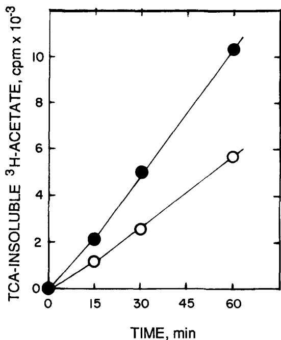
Figure 8. Acetylation of tubulin dimer and polymer. The time course of PC tubulin (1.4 mg/ml) acetylation, with 0.13 mg/ml MAPs (●) (tubulin polymers) or without MAPs (tubulin dimers) (○), was followed in the presence of 0.28 units of NaCl extract of the flagellar axonemes.
