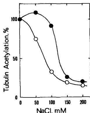
Figure 1. Effect of salt on tubulin acetylation. Acetylation of brain MTP was measured for 60 min at various concentrations of NaCl, as indicated, with 0.14 units of axonemal bound (detergent-insoluble; ●) or free (0.66 M NaCl-soluble; ○) TAT preparations (for the definition of TAT unit, see Table I). 100% activity corresponds to 0.4 acetate per tubulin dimer (mol/mol) per hour.
