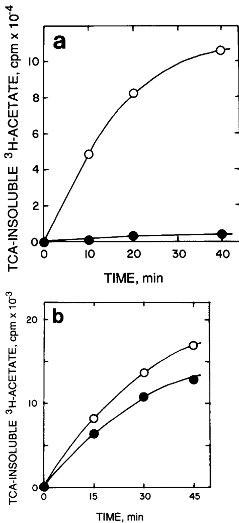
Figure 4. Effect of Ca 2+ on acetylation of tubulin dimers and histones. (a) The time course of the acetylation of PC tubulin (1.4 mg/ml) without MAPs was followed in the presence (●) and absence (○) of 1 mM Ca 2+ . (b) The time course of the acetylation of histones (7.0 mg/ml) was followed in the presence (●) and absence (○) of 1 mM Ca 2+ . In both cases 0.14 units of the same NaCl extract of flagellar axonemes were used as an acetyltransferase source. Note that the concentration of histone (a poor substrate) was five times higher than that of tubulin dimer and that there is a 10-fold difference in the ordinates (acetyltransferase activity) for tubulin compared with those for histone.
