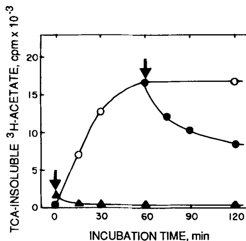
Figure 7. TAT inhibitor and TDA activities of Chlamydomonas cell body extract. (○) Brain MTP was acetylated by Chlamydomonas flagella over 60 min, at which point, the supply of ^3\text{H} -acetyl CoA was completely exhausted. (▲) To assay for cytoplasmic TAT inhibitor activity, Chlamydomonas cell body extract was added to the TAT assay mixture at 0 min (arrow). (●) To assay for cytoplasmic TDA activity, Chlamydomonas cell body extract was added to the TAT assay mixture at 60 min, as a second arrow indicates. For details, see the text.
