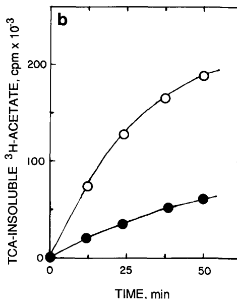
Figure 9(a). Effect of colchicine on acetylation of tubulin dimer and polymer. Acetylation of PC tubulin (1.4 mg/ml) by 0.14 units of NaCl extract of the flagellar axonemes was measured for 60 min at various concentrations of colchicine, as indicated, without (○) or with (●) MAPs (0.13 mg/ml). (b) Effect of taxol on acetylation of microtubules. Acetylation of PC tubulin (14 μM) with MAPs (0.13 mg/ml) by 0.14 units of NaCl extract of the flagellar axonemes was measured over 50 min, in the presence (●) or absence (○) of 20 μM taxol.
