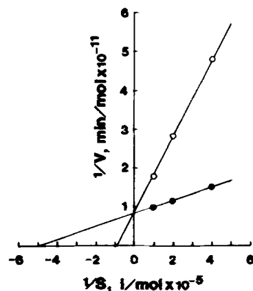
Figure 6. Determination of K_m and K_i for acetyl CoA and its competitive inhibitor CoA. The rate of tubulin acetylation by TAT-2 was measured at various concentrations of ^3\text{H} -acetyl CoA in the presence (○) or absence (●) of 24 \mu\text{M} CoA.
