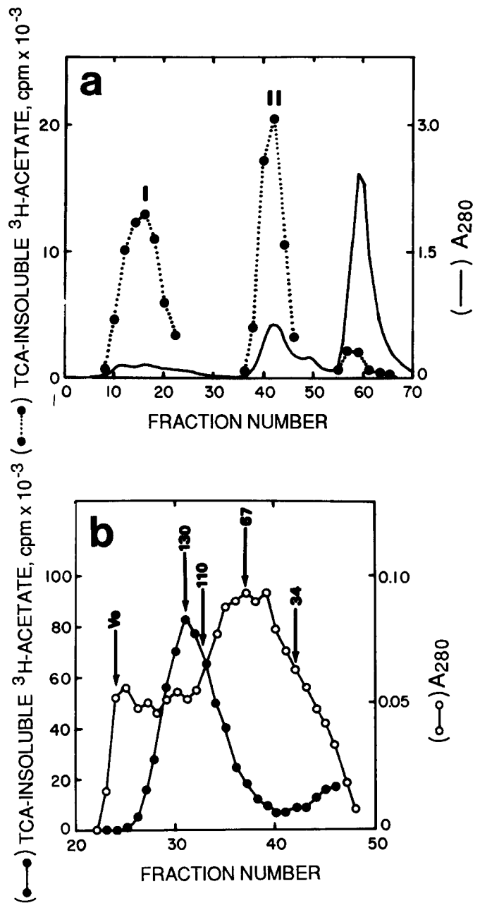
Figure 5. DEAE-cellulose chromatography (a) and gel-filtration on Sephadex G-150 (b) of the axonemal TATs. (a) 20 ml of NaCl extract of the flagellar axonemes after dialysis against TDSA buffer was applied to DE-52 (bed vol 20 ml) equilibrated with TD buffer and the bound proteins were eluted by a stepwise gradient of NaCl (50 and 400 mM). 10 \mu l of each fraction was assayed for TAT activity for 60 min under the standard conditions. Peaks I and II of TAT activity correspond to the flow-through and 50 mM NaCl eluate fractions, respectively. (b) 50 mM phosphate eluate from hydroxylapatite of NaCl extract of the flagella was further fractionated on Sephadex G-150. The TAT activity of each fraction was measured as described in Fig. 5 a. The arrows indicate molecular weights of standard proteins.
