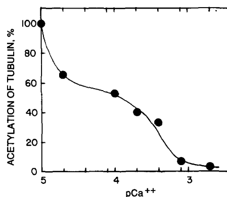
Figure 3. Effect of Ca^{2+} on tubulin acetylation. Acetylation of brain MTP (1.4 mg/ml) was measured for 60 min at various concentrations of Ca^{2+} , as indicated, with 0.35 units of NaCl extract of flagellar axonemes.
