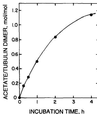
Figure 2. Stoichiometry of tubulin acetylation. The time course of tubulin acetylation using in vitro-assembled brain MTP (25 \mu M) as a substrate was followed in the presence of 0.28 units of NaCl extract of flagellar axonemes as a TAT source.
