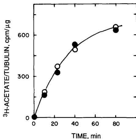
Figure 12. Acetylation of alpha-tubulin in preparations of control and sheared microtubules. The time course of tubulin acetylation of the control and sheared microtubules (see Fig. 11) was followed at 37°C in the presence of NaCl extract of the flagellar axonemes and ^3\text{H} -acetyl CoA as described under Materials and Methods. After the indicated time of incubation, each sample was centrifuged in an airfuge, and the microtubules in each pellet were subjected to SDS/urea PAGE and the radioactivity in each alpha-tubulin band was measured as described under the Materials and Methods. ●, control microtubules; ○, sheared microtubules.
