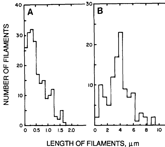
Figure 11. Length distribution of sheared and control microtubules. Calf brain microtubules were mechanically sheared, fixed with glutaraldehyde, and negatively stained as described under Materials and Methods. The length of the sheared microtubules was compared with the control microtubules by electron microscopy. (A) Sheared microtubules, the average length of ~200 filaments was 0.6 \mu\text{m} . (B) Control microtubules, the average length of 100 filaments was 3.4 \mu\text{m} .
