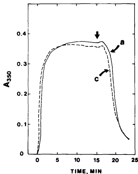
Figure 10. Time course of polymerization and depolymerization of the acetylated and nonacetylated (control) tubulins. The acetylated (a) and control (c) tubulin dimer preparations (0.8 mg/ml), obtained after one additional cycle of temperature-dependent polymerization/depolymerization as described under Materials and Methods, were incubated at 37°C in the presence of 0.3 M glycerol and 2 mM EGTA for in vitro polymerization. After 15 min, as indicated by the arrows, the temperature was shifted to 4°C to initiate depolymerization. The time courses of both polymerization and depolymerization were followed by monitoring the turbidity changes at 350 nm.
