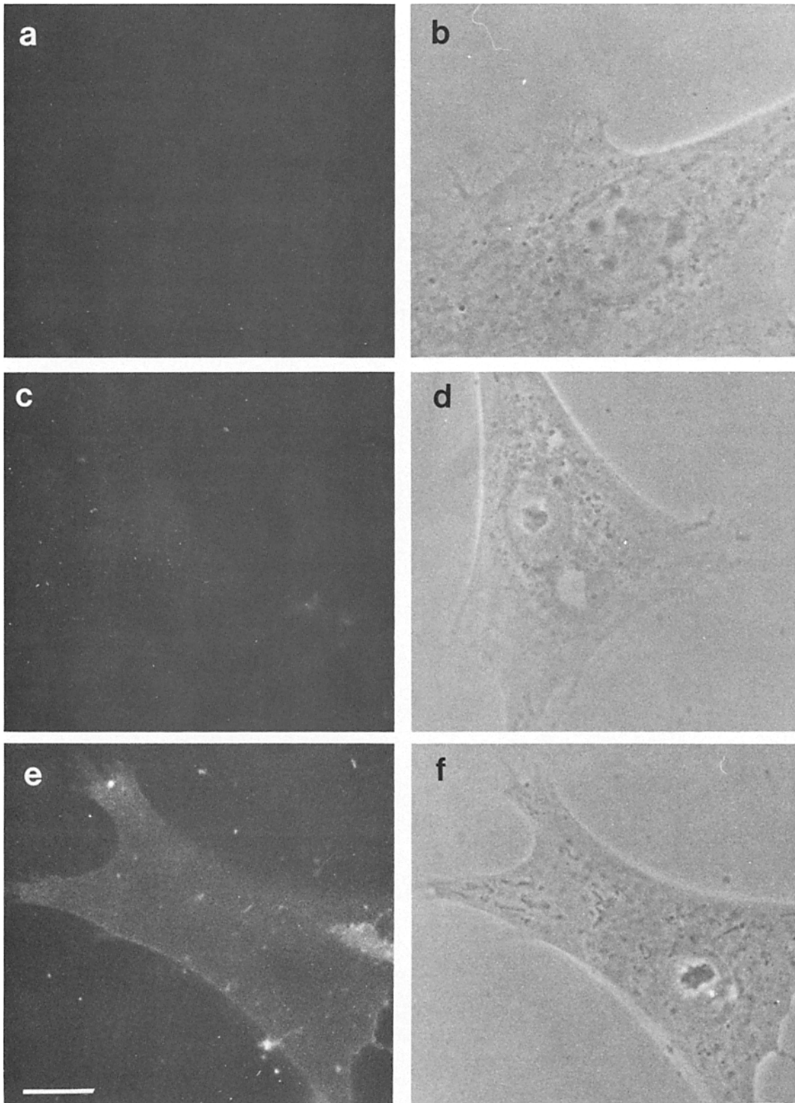
Figure 9. Sensitized acceptor fluorescence in BHK cells labeled with FITC-LCA and (C 6 -SRh)-PC. ( a and b ) Cells were incubated with 30 μg FITC-LCA/ml for 30 min at 2°C. ( c and d ) Cells incubated with 2 μM (C 6 -SRh)-PC for 30 min at 2°C. ( e and f ) Cells were co-incubated with FITC-LCA and 2 μM (C 6 -SRh)-PC for 30 min at 2°C. ( a , c , and e ) Fluorescence in transfer channel; ( b , d , and f ) phase-contrast micrograph. Exposure time and processing for a , c , and e were identical. Bar, 10 μm.
