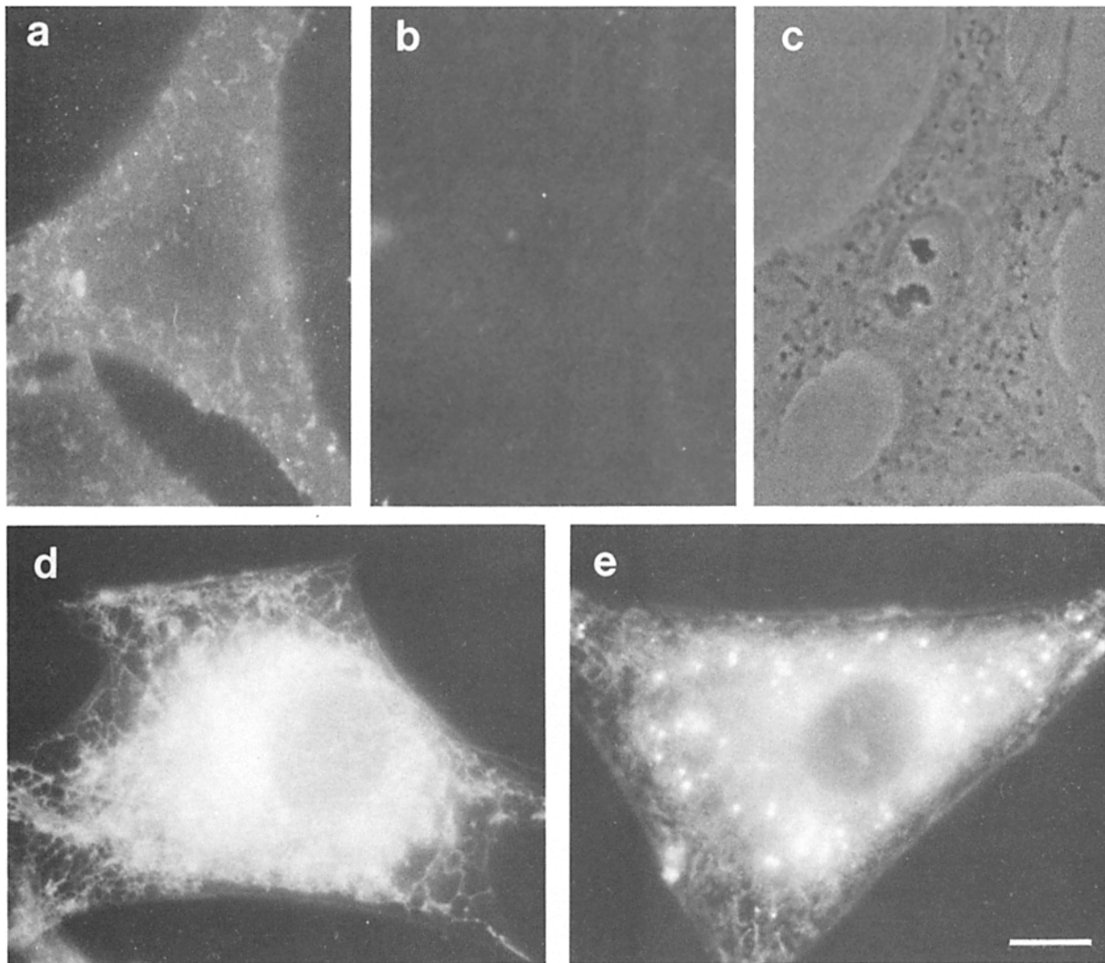
Figure 5. Cellular labeling of BHK fibroblasts with fluorescent lipophilic probes. (a) Cells incubated with 2 \mu\text{M} (\text{C}_6\text{-SRh})\text{-PC} for 30 min at 2°C. (b) (\text{C}_6\text{-SRh})\text{-PC} labeled cells after three successive incubations with 0.1 mM DOPC liposomes for 15 min at 2°C, and photographed under similar conditions as in a. (c) Phase-contrast micrograph of the field in b. (d) Cells incubated with 1 \mu\text{g} N\text{-SRh-C}_{10} /ml for 8 min at 37°C. (e) Cells incubated with 100 \mu\text{M} (\text{C}_6\text{-NBD})\text{-PA/DOPC} (4:6) liposomes for 1 h at 2°C, washed, and warmed for 15 min at 37°C. (a, b, and d) Fluorescence in acceptor channel; (e) fluorescence in donor channel. Bar, 10 \mu\text{m} .
