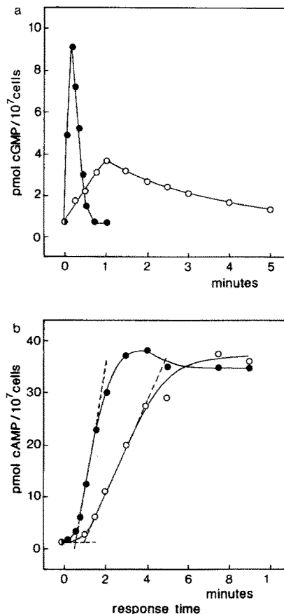
Figure 1. cGMP response (a) and cAMP response (b) at 20 (●) and 0°C (○). (a) Aggregative D. discoideum cells ( 5 \times 10^7 cells/ml) were stimulated with 0.1 \mu M cAMP. At the times indicated 20 \mu l of the cell suspension was added to 20 \mu l perchloric acid (3.5%, vol/vol). The lysates were neutralized, and the cGMP content was measured by radioimmunoassay. (b) Cells were stimulated with 10 \mu M dcAMP and 5 mM DTT, and lysed with perchloric acid at the times indicated. The cAMP content was measured with a binding protein assay. The results shown are the means of duplicate determinations in an experiment reproduced four times.
