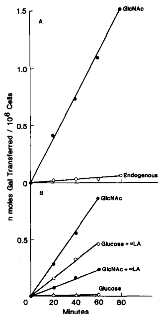
Figure 1. Intact B16-F10 melanoma cells have abundant surface GalTase activity. (A) Activity towards soluble exogenous substrates (●) is >25 times higher than activity towards cell-bound endogenous substrates (○). (B) α-LA lessens the activity of surface GalTase on B16-F10 melanoma cells for its conventional substrate, GlcNAc (●), and increases it for glucose (○), a substrate of normally low affinity.
