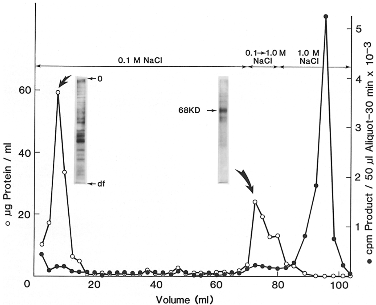
Figure 7. Differential elution of distinct laminin binding proteins from laminin affinity columns. Detergent-solubilized B16-F10 plasma membranes were applied to a laminin affinity column as described in Materials and Methods. After washing away unbound protein, a salt gradient eluted the 68-kD receptor, as well as other laminin-binding proteins, at 0.2–0.3 M NaCl. GalTase eluted at 1.0 M NaCl as assayed by enzymatic activity. The eluted protein was resolved by silver stained SDS-PAGE, and representative fractions are illustrated. GalTase has an apparent molecular mass of 60 kD by immunoblot analysis.
