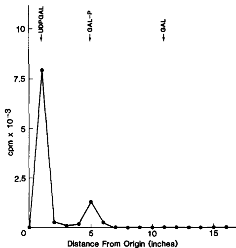
Figure 2. Hydrolysis of UDPGal during B16-F10 melanoma surface GalTase assays. At the end of the incubation, there is no detectable pool of free, radiolabeled galactose.
