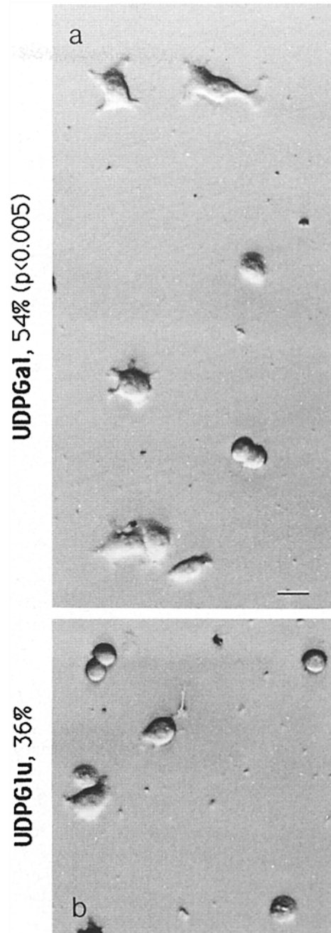
Figure 5. Cell spreading on laminin is accelerated by UDPGal. (a) UDPGal increases cell spreading (304 cells scored) relative to controls containing the inappropriate sugar nucleotide UDPGlu (b; 290 cells scored). The presence of UDPGlu has no significant effect on cell spreading relative to no sugar nucleotide addition (92% of control, P > 0.4 ). All photographs were taken after 1½ h of culture. After cells are fully spread (i.e., by 4 h of incubation), UDPGal no longer facilitates cell spreading. The percentages of cells spread in the presence of 20 mM sugar nucleotide are shown; 5 mM sugar nucleotide produced similar results. This experiment was repeated six times with similar results. Bar, 10 \mu m.
