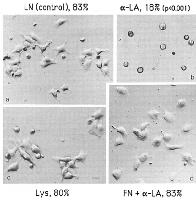
Figure 3. Cell spreading on laminin, but not cell adhesion, is inhibited by the GalTase substrate modifier protein, \alpha -LA. (a) Cells on laminin (control; 310 cells scored); (b) 5 mg/ml \alpha -LA inhibits cell spreading, but not cell adhesion (437 cells scored); (c) 5 mg/ml of the structurally similar protein, lysozyme, has no effect (350 cells scored); (d) 5 mg/ml \alpha -LA has no effect on cell spreading on fibronectin (360 cells scored). All photographs were taken after 4 h of culture. The percentages of cells spread are shown. This experiment was repeated three times with similar results. In all photographs, a fine granularity on the laminin surface is evident by Hoffman modulation optics. Bar, 10 \mu m.
