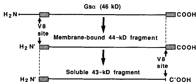
Figure 8. Schematic mapping of the V8 protease cleavage sites on G \alpha long form. The hatched bars indicate the location of the amino acid sequences which are recognized by the NH 2 -terminal antiserum and the COOH-terminal antiserum.
