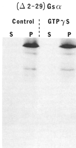
Figure 7. Membrane association of ( \Delta 2-29 )G \alpha . T7 polymerase transcription products were translated in reticulocyte lysate with ^{35}\text{S} -methionine and cyc - membranes were reconstituted with the translation medium as described in Materials and Methods. Reconstitution of cyc - membranes by in vitro-translated ( \Delta 2-29 )G \alpha was performed as described in Materials and Methods. Reconstituted membranes were incubated for 10 min at 37°C in the absence or the presence of 100 \mu\text{M} GTP \gamma S and 10 mM MgCl 2 and then centrifuged at 10,000 g for 5 min. The supernatant and the pellet fractions were processed as described previously (13). The ^{35}\text{S} -labeled proteins were resolved on a 9% acrylamide gel as shown previously (16) and visualized by autoradiography.
