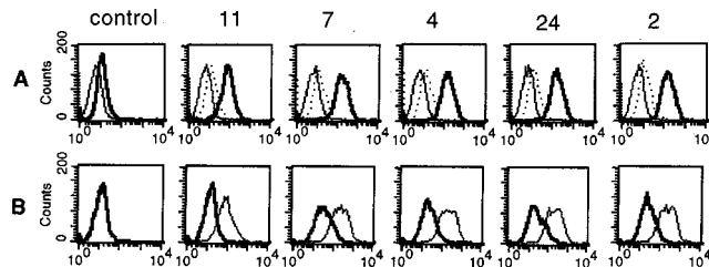
FIG. 3. Flow cytometry histograms demonstrating that humanized LM609 binds specifically to human integrin α v β 3 and can be blocked by mouse LM609. (A) Binding of humanized LM609 Fab to untransfected CS-1 hamster cells (fine line) and CS-1 hamster cells transfected with either human β 3 (bold line) or β 5 cDNA (dotted line). (B) Binding of humanized LM609 Fab to CS-1 hamster cells transfected with human β 3 cDNA in the presence of a fourfold molar excess of mouse AP3 IgG (fine line) or mouse LM609 IgG (bold line). Clones 11, 7, 4, 24, and 2 represent the five humanized LM609 versions (cf. Fig. 2). Controls in A and B are based on identical experiments using buffer instead of humanized LM609 Fab. The y axis gives the number of events in linear scale, the x axis the fluorescence intensity in logarithmic scale.
