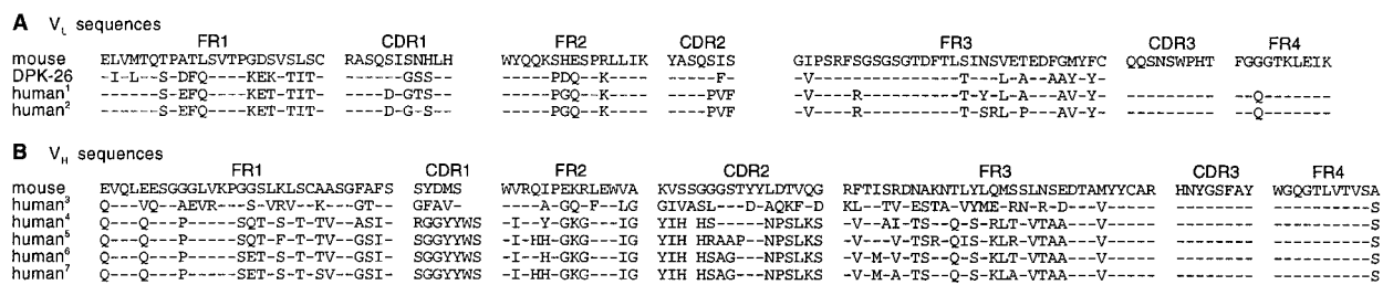
FIG. 2. Amino acid sequence alignment of mouse and humanized LM609. Shown are FRs and CDRs. Dashes indicate identical amino acids. Note that due to our grafting procedure CDR3 is identical in the original mouse and the selected human sequences. (A) Alignment of the selected human V L sequences. Databank screening revealed that the two selected human V L sequences are derived from germ-line DPK-26 of the V κ 3 family. (B) Alignment of the selected human V H sequences. Five different human V H sequences were selected. Four of them, represented by clones 7, 4, 24, and 2, are highly related in amino acid sequence; they share an identical V L domain and an amino acid sequence identity of at least 85% in their V H domains. The V H sequences are all derived from germ-line DP-65 or the highly related DP-78. In contrast, clone 11 represents a humanized version with a V H domain that is derived from a different germ-line family. This humanized version also contains a different V L domain which is 96% identical and derived from the same germ-line. Germ-lines were determined by nucleic acid sequence alignment using DNAPLOT software provided by the VBASE Directory of Human V Gene Sequences ( http://www.mrc-cpe.cam.ac.uk/imt-doc/ ). 1 clone 11, germ-line DPK-26 (V κ 6 family); 2 clones 2, 4, 7, 24, germ-line DPK-26 (V κ 6 family); 3 clone 11, germ-line DP-10 (V H 1 family); 4 clone 7, germ-line DP-78 (V H 4 family); 5 clone 4, germ-line DP-65 (V H 4 family); 6 clone 24, germ-line DP-65 (V H 4 family); 7 clone 2, germ-line DP-65 (V H 4 family).
