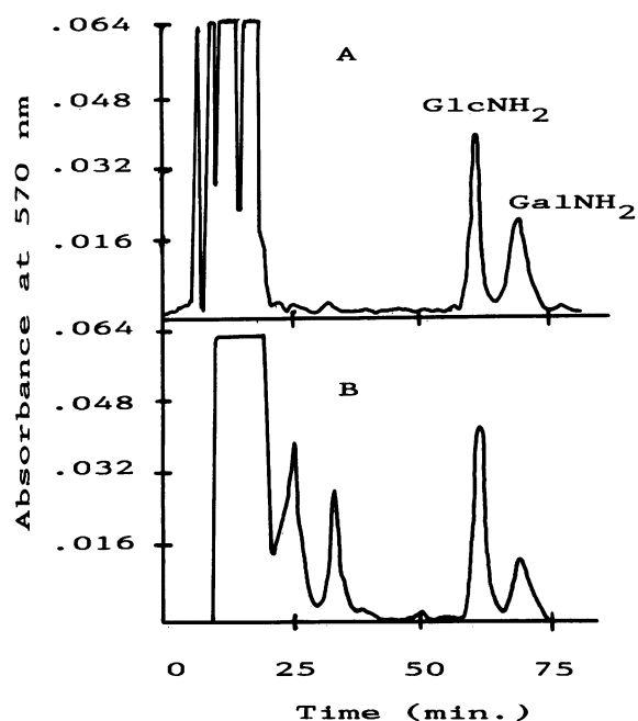
FIG. 1. Chromatographic separation of amino sugars on an amino acid analyzer. (A) Amino acid calibration mixture (500 nmol) plus 10 \mu g of both glucosamine and galactosamine per ml; (B) analysis of 0.5 mg of B. thuringiensis subsp. israelensis crystal protein after hydrolysis in 4 N HCl for 6 h. Abbreviations: GlcNH 2 , glucosamine; GalNH 2 , galactosamine.
