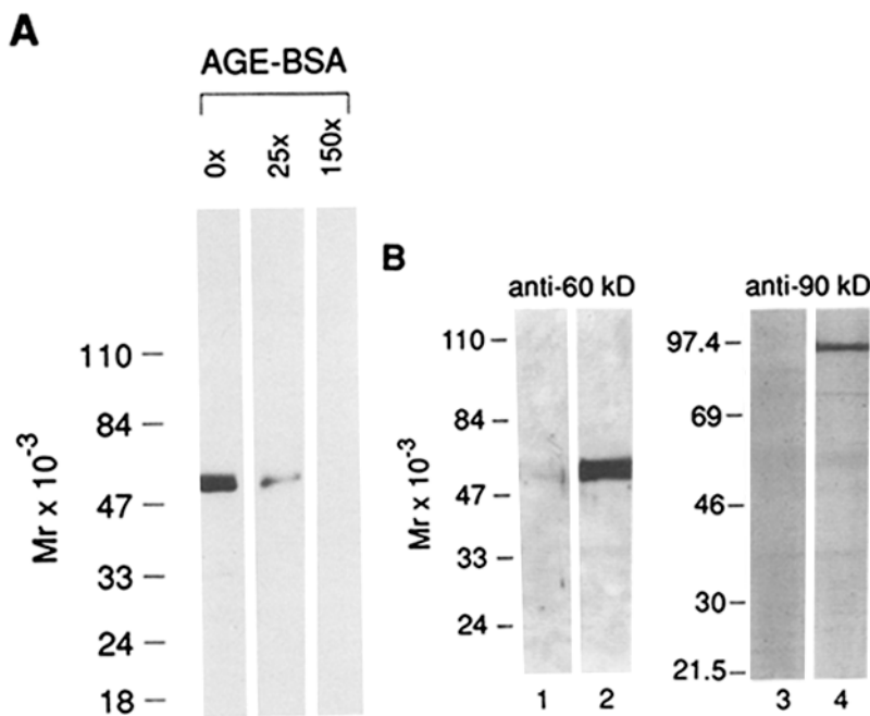
Figure 4. (A) Ligand blot analysis of rat liver membrane proteins. Aliquots (15 \mu\text{g} each) of detergent-solubilized membrane proteins were subjected to electrophoresis through 8–16% acrylamide gradient gel under nonreducing conditions and electro-transferred onto nitrocellulose filters. Using ^{125}\text{I} -AGE-BSA (50 nM, 8.0 \times 10^5 cpm/ng) as probe, specific binding was determined in the presence of 0-, 25-, or 150-fold excess nonlabeled AGE-BSA using autoradiographic detection. Migration of molecular mass standards is shown at left. (B) Aliquots of solubilized membrane proteins (mercaptoethanol reduced), were subjected to electrophoresis through an 8–16% gradient gel and electro-transferred onto nitrocellulose filters. After washing and blocking with excess BSA, the blots were probed with purified IgG fractions of either anti-p60 or anti-p90 chicken antisera or the corresponding preimmune sera, and then exposed to goat anti-chicken antibody conjugated to alkaline phosphatase and reacted for phosphatase-dependent color development. Lane 1, preimmune IgG; lane 2, anti-p60 IgG; lane 3, preimmune IgG, lane 4, anti-p90 IgG. Results are representative of three independent experiments.
