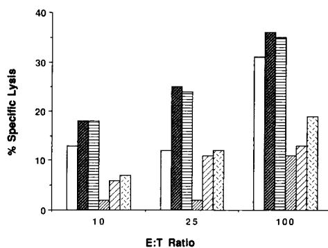
Figure 4. ADCC of HuG1-M195 and Hd-IgG is shown as a function of concentration and E/T ratio. Target HL60 cells were incubated at 37°C with mAb and PBMC as effectors, and 51 Cr-release was measured 5-h later as described in the text. Hd-IgG was 100-fold more potent (50 times on a weight basis) and 2–6 times more effective than the HuG1-M195 at ADCC. Hd-IgG at 0.2 µg/ml (▨); Hd-IgG at 1 µg/ml (■); Hd-IgG at 10 µg/ml (≡); HuG1-M195 at 0.2 µg/ml (▩); HuG1-M195 at 1 µg/ml (⊞); HuG1 at 10 µg/ml (⊠). Results shown are from a representative experiment that was repeated on three separate days.
