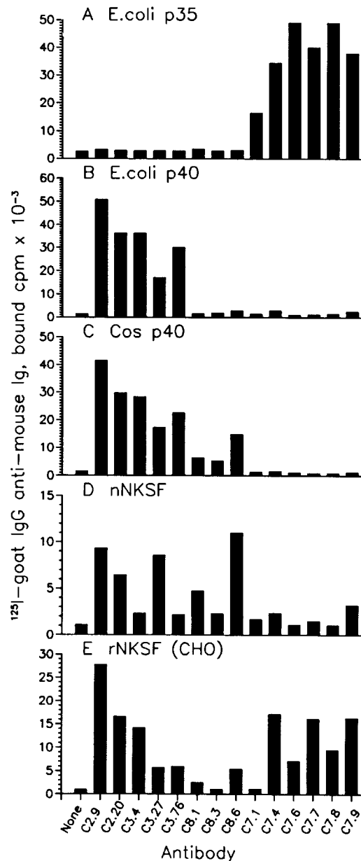
Figure 1. Indirect RIA of representative anti-NKSF/IL-12 mAb tested against various preparations of NKSF/IL-12 or its free chains. Purified E. coli -derived p35 chain (A), E. coli -derived p40 chain (B), Cos-derived p40 chain (C), semipurified RPMI 8866-derived nNKSF/IL-12 (both p40 and p70) (D), and pure CHO-derived rNKSF p70 heterodimer (E) were adsorbed to 96-well vinyl plates, and binding of the indicated mAb was detected with a second ^{125}\text{I} -labeled affinity-purified goat antibody anti-murine Ig.
