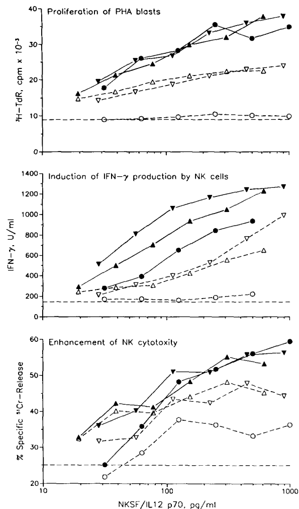
Figure 7. Biological activity of SAC-induced NKSF/IL-12 produced by PBMC. PBMC from healthy donors A and B were cultured ( 10^6 cells/ml, 1% FCS, 18 h at 37^\circ\text{C} ) in the presence of 0.0075% SAC, supernatant fluids were collected, and concentrated 10-fold. The concentration of the p70 heterodimer, as determined by RIA, in 10-fold concentrated supernatant fluids from donors A and B, were 1.8 and 1.2 ng/ml, respectively. Twofold dilutions of the concentrated fluids were then tested for their ability to induce proliferation of PHA blasts ( [^3\text{H}]\text{TdR} incorporation, 48-h cultures), induction of IFN- \gamma production by purified NK cells ( 5 \times 10^6 cells/ml, 18-h cultures, in the presence of 100 U/ml rIL-2), and enhancement of NK cell-mediated cytotoxicity. 2 \times 10^5 PBL were incubated for 18 h in round-bottomed 96-well plates in the presence of dilutions of supernatant fluid or rNKSF/IL-12 and in the presence of anti-IFN- \alpha , anti-IFN- \beta , and anti-IL-2 antibodies; ^{51}\text{Cr} -labeled Daudi cells were then added ( 10^4 /well) and supernatant fluid for determination of ^{51}\text{Cr} -release were collected after 3 h. All experiments were performed in the presence (dashed lines and open symbols) or absence (solid lines and filled symbols) of anti-NKSF/IL-12 antibodies C8.6 and C8.1 ( 10 \mu\text{g}/\text{ml} each). The continuous horizontal dashed line indicates the control values in the absence of supernatant fluids or rNKSF/IL-12. (● and ○) rNKSF/IL-12; (▼ and □) supernatant fluid of donor A; (▲ and △) supernatant fluid of donor B.
