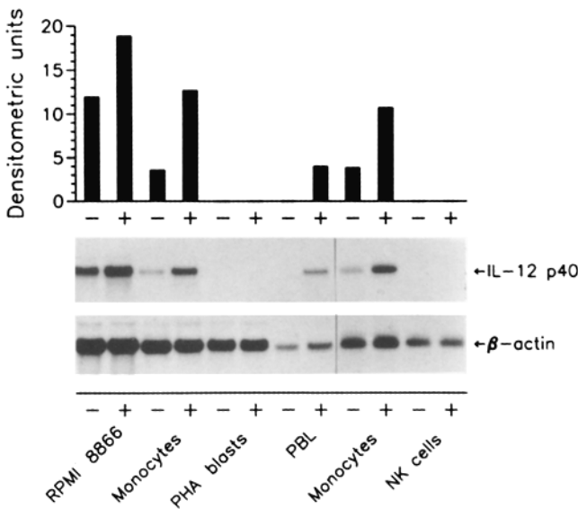
Figure 5. The accumulation of NKSF/IL-12 p40 mRNA is enhanced by phorbol diester stimulation of the RPMI 8866 cell line and by SAC stimulation of adherent PBMC and PBL. Total RNA was extracted from RPMI 8866 unstimulated (-) or stimulated with 10^{-7} M PDBu (+) and from two preparations of plastic-adherent PBMC (indicated as Monocytes in the figure and containing >95% CD14 + cells) and one preparation of monocyte-depleted PBL, PHA blasts, and NK cells unstimulated (-) or stimulated with 0.0075% (wt/vol) SAC(+). The Northern blot was hybridized with 32 P-cDNA for p40 NKSF/IL-12 and for \beta -actin. For densitometric analysis of the hybridization with p40 cDNA ( top ), the values of the induced and uninduced cells are corrected according to the relative intensity of \beta -actin hybridization.
