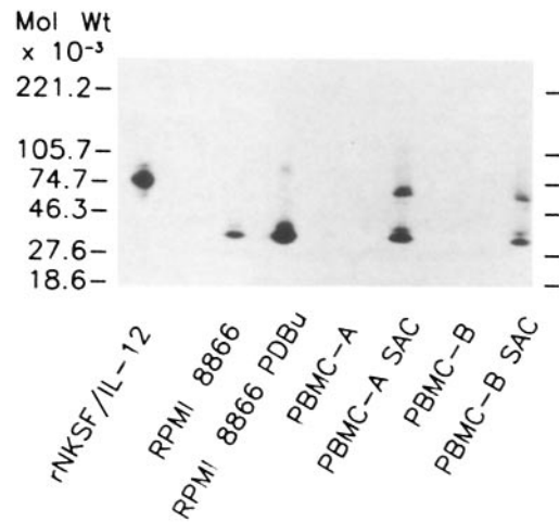
Figure 6. Western blotting analysis of recombinant and natural NKSF/IL-12. Western blotting was performed as described using 1 ng CHO cell-derived rNKSF/IL-12 and immunoprecipitates with antibody C11.79 (anti-p40) from the supernatant fluid (1 ml, 10-fold concentrated) of RPMI 8866 cells, stimulated or not with 10^{-7} M PDBu, or of PBMC from two donors (A and B), stimulated or not with 0.0075% SAC. 125 I-labeled antibody C8.6 was used for detection of the blotted NKSF/IL-12. The supernatant fluids from SAC-stimulated PBMC from donors A and B were the same as those used for the experiments in Fig. 7.
