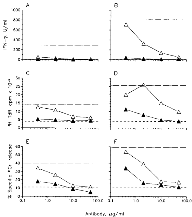
Figure 2. Ability of anti-NKSF/IL-12 mAb to neutralize rNKSF/IL-12 biological activities. The indicated concentrations of purified IgG1 mAbs C8.1 ( \Delta ) and C8.6 ( \blacktriangle ) were added to rNKSF/IL-12 (0.2 ng/ml, A, C, and E; 1 ng/ml, B, D, and F), and the ability of rNKSF/IL-12 to induce IFN- \gamma production from PBL (A and B), induce proliferation of PHA blasts (C and D), and enhance PBL-mediated spontaneous cytotoxicity of Daudi-target cells (E/T cell ratio of 50:1, E and F) was tested as described. In each panel the dashed line indicates the activity of cells not treated with rNKSF/IL-12, and the dash-dot-dash line indicates the activity of cells treated with rNKSF/IL-12 in the absence of mAb.
