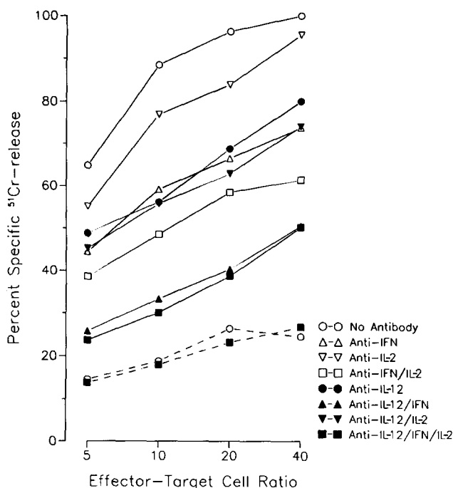
Figure 8. NK cell-mediated cytotoxicity-enhancing activity of SAC-induced supernatant fluid from PBMC. PBL from a normal donor were cultured ( 5 \times 10^6 cells/ml, 18 h, 37^\circ\text{C} ) in medium (dashed lines) or in the presence (solid lines) of supernatant fluids from SAC-stimulated PBMC (same donor A as in Figs. 6 and 7) at a dilution corresponding to a concentration of 0.3 ng/ml NKSF/IL-12 p70. The following antibodies were present during the culture: (○ and ●) no antibody; (△ and ▲) sheep anti-IFN- \alpha (1:200) and cow anti-IFN- \beta (1:200); (□ and ▼) goat anti-IL-2 (1:200); (□ and ■) anti-IFN and anti-IL-2. Open symbols refer to cultures in the absence, and filled symbols to cultures in the presence, of anti-NKSF/IL-12 C8.6 and C8.1 antibodies ( 10 \mu\text{g}/\text{ml} each). PBL were then washed and tested at the indicated E/T cell ratio against ^{51}\text{Cr} -labeled Daudi target cells in a 3-h cytotoxic assay.
