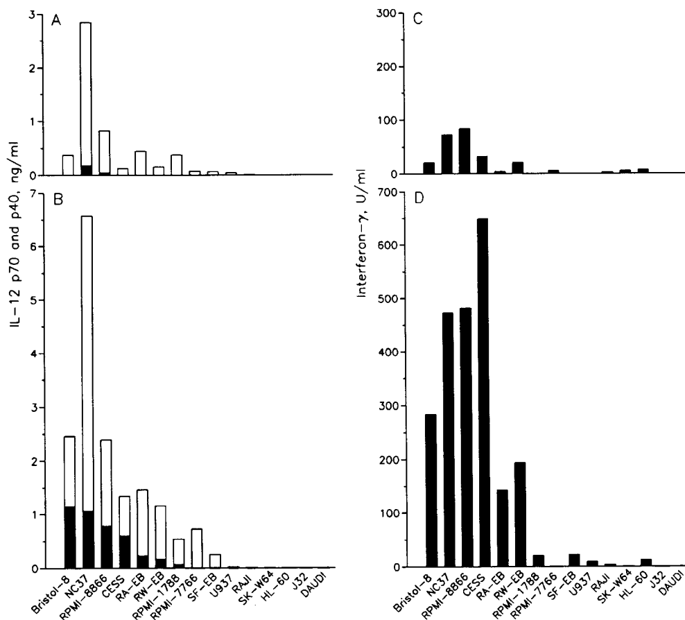
Figure 4. Constitutive and phorbol diester-induced production of free p40 chains and biologically active p70 heterodimers by human cell lines. Cell-free supernatant fluids from the indicated cell lines were obtained after an 18-h incubation in the absence (A and C) or presence (B and D) of 10^{-7} M PDBu. The concentration of the p70 heterodimer (C11.5/ ^{125} I-20C2 RIA, filled portion of the bars, A and B) and of the free p40 chain (C8.3/ ^{125} I-C8.6 RIA, open portion of the bars) was determined. For determination of IFN- \gamma -inducing activity (C and D), the supernatant fluids (after extensive dialysis of those containing PDBu) were added at dilutions of 1:2 to purified NK cells (blasts) in the presence of 100 U/ml rIL-2. The values reported are the difference between IFN- \gamma production in the presence and in the absence of 10 \mu g/ml C8.6 neutralizing anti-NKSF/IL-12 mAb.
