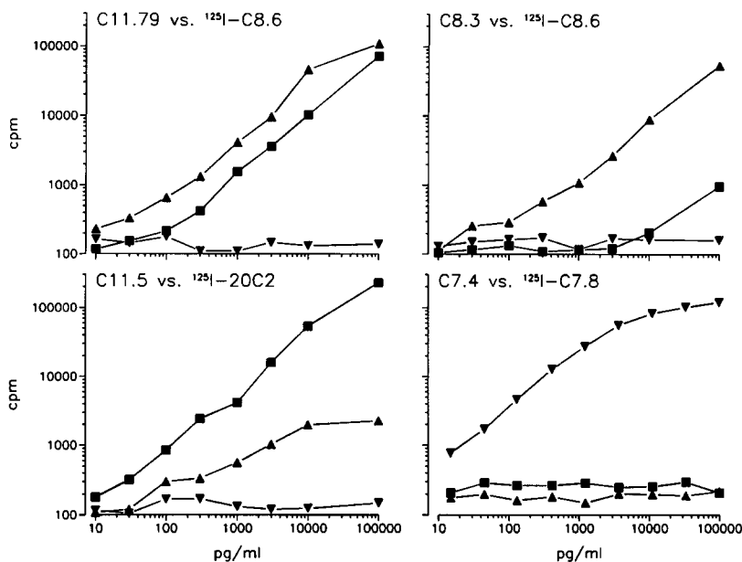
Figure 3. Double determinant RIAs with anti-NKSF/IL-12 antibodies. The indicated different pairs of mAbs were used in RIA as described using as standards purified CHO-derived p70 NKSF/IL-12 heterodimer ( \blacksquare ), Cos-derived p40 ( \blacktriangle ), and E. coli -derived p35 ( \blacktriangledown ).
