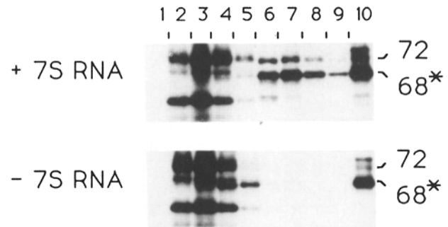
Figure 3. Assembly of SRP72 with SRP68 into a ~9S particle requires the presence of 7S RNA. In vitro synthesized SRP72 and SRP68* (shortened from the COOH-terminus by 24 amino acids; see Fig. 4b) were separated by centrifugation through sucrose gradients as in Fig. 2 (lower left and middle panels) and recovered from fractions 2–4 (SRP72) or the pellet fraction (SRP68*). Subsequently they were mixed with reticulocyte lysate which had been absorbed twice to an equal volume of DEAE-Sephacel and incubated in the presence (upper panel) or absence (lower panel) of purified 7S RNA. Resulting complexes were analyzed by sucrose gradient centrifugation as in Fig. 2.
