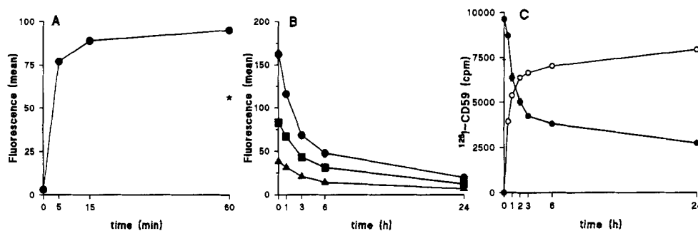
Figure 1. FACscan analysis of CD59 incorporated into U937. (A) U937 cells were incubated with 5 \mu\text{g/ml} CD59 for various periods of time, washed, and stained for CD59 (●). ★, level of expression of CD59 in the CD59 positive subline (van den Berg et al., 1994). (B) U937 cells were incubated with CD59 (●: 15, ■: 5, ▲: 1.5 \mu\text{g/ml} ) for 10 min. Cells
