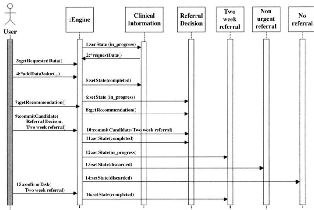
Figure 5. Sequence diagram shows the use of the guideline shown in Figure 4.
