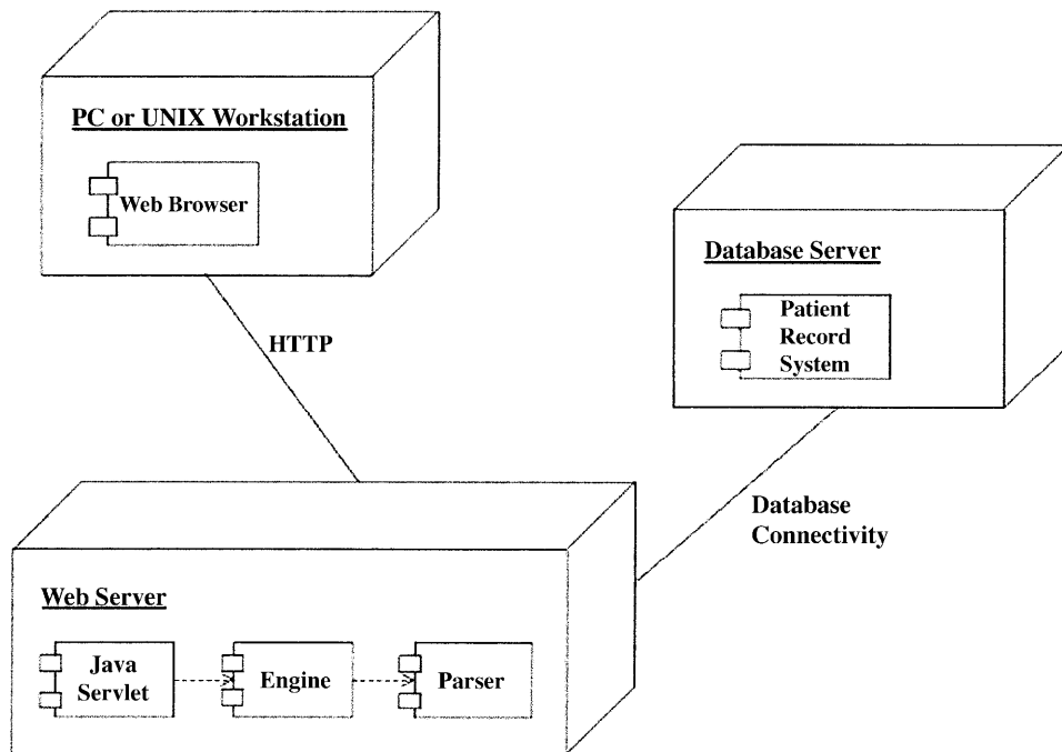
Figure 3. Deployment of Tallis components when enacting a guideline over the Web.
