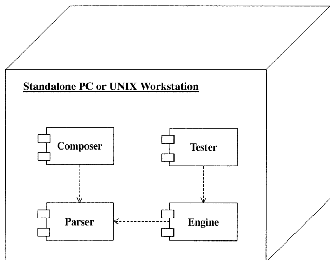
Figure 2. Deployment of Tallis components in the guideline development environment.
