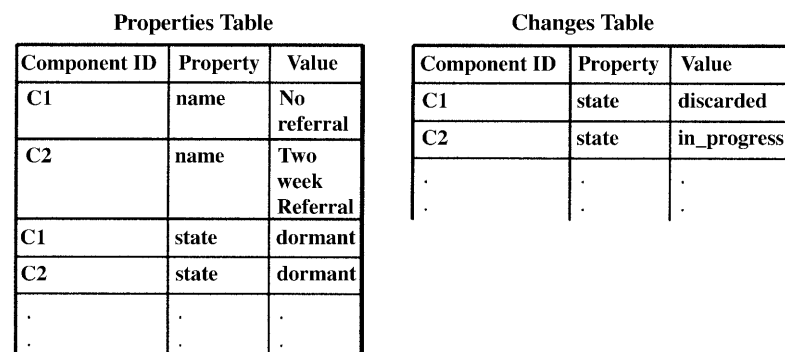
Figure 8. Example of engine state.
