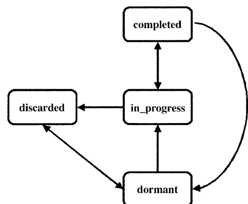
Figure 7. Task state transitions. An arrow between two states indicates that a transition between those states is possible. The circumstances in which the transition would actually occur are too complex to show in the diagram.
