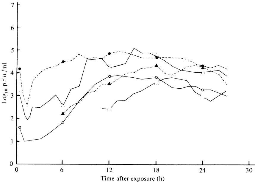
Fig. 3. Pharyngeal virus growth curves from five cattle exposed to various doses of foot-and-mouth disease virus, type 0. PFU of virus/l of air: ●, 10^{5.8} ; ▲, 10^{2.8} ; ○, 10^{3.8} ; ■, 10^{1.8} ; □, 10^{0.8} .
