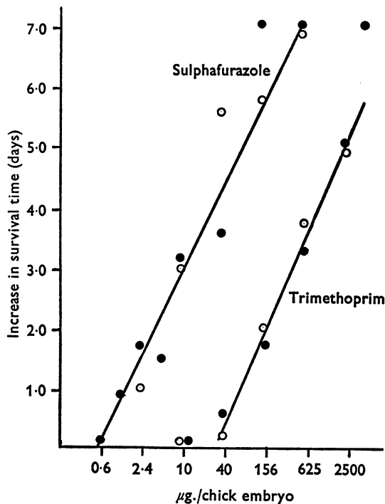
Fig. 2. Effect of sulphafurazole and trimethoprim on the survival of chick embryos inoculated with strain T'ang, ○, or strain MRC-4, ●. Chick embryos hatched if the survival time was extended beyond about 7 days.
