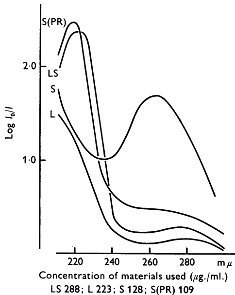
Fig. 1. Ultraviolet absorption spectra of LS, L, S, S(PR).
