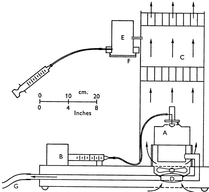
Fig. 2. Airborne particle generator. A, Spinning top (May, 1949); B, mechanically driven syringe for feeding suspension; C, vertical wind-tunnel with baffles to reduce turbulence; D, fan; E, sedimentation chamber for sampling dispersal cloud; F, sampling plate for cloud; G, tube to lead effluent air from spinning top, with satellite particles, out of room.
