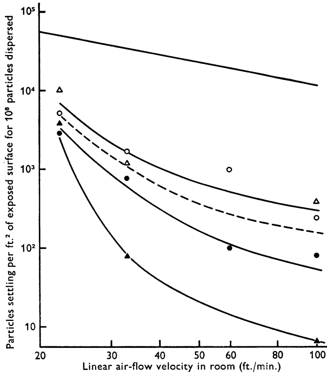
Fig. 4. Transfer across the direction of air flow. Dispersal took place at point A in area B 1. Triangular symbols, \Delta and \blacktriangle , record experiments in which movement was restricted to the rear and area B 1 only (coded 2 in text and Table 1). Circular symbols, \circ and \bullet , record experiments in which movement extended over the whole of the room area (coded 3 in text and Table 1). Open symbols, \Delta and \circ , record the spore-bearing particles recovered from the six plates exposed in area B 2, close to the centre-line of the room. Filled symbols, \blacktriangle and \bullet , record the spore-bearing particles recovered from the remaining six plates exposed in area B 2 close to the wall of the room. The upper straight line shows the numbers of spore-bearing particles that would have been recovered if the air had been completely mixed by turbulent movements. The lower curves have been drawn in by eye to illustrate the effect of the various conditions on the number of spore-bearing particles recovered.
