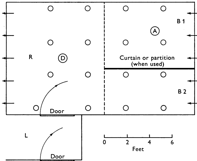
Fig. 3. Plan of room. B 1, B 2, Notional bed areas; R, rear area of room downwind of bed areas. A, dispersal point in B 1; D, dispersal point at rear of room. The unlabelled circles mark the position of the sixteen stands each carrying up to three 5½ in. diameter Petri dishes (F in Fig. 1).
