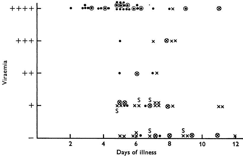
Fig. 1. Viraemia in haemorrhagic smallpox patients. ●, Type I; ×, type II; ⊙, ⊗, unvaccinated, type I or type II; S, survived.
