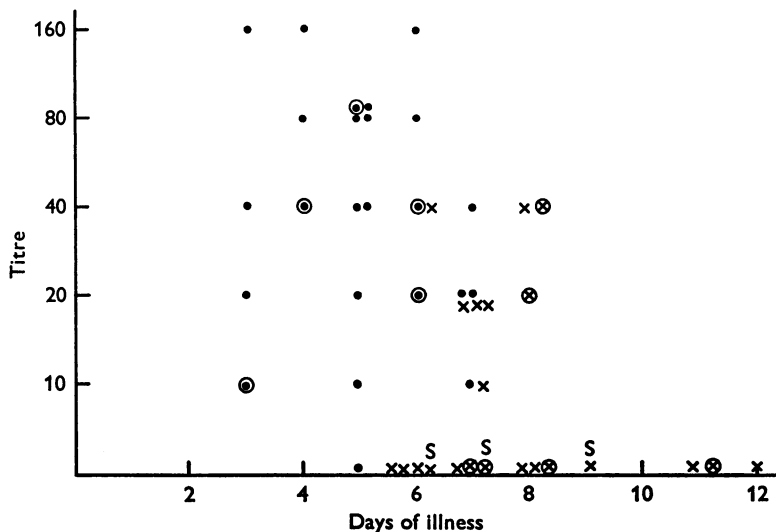
Fig. 2. Antigen in serum of haemorrhagic smallpox patients. ●, Type I; ×, type II; ⊙, ⊗, unvaccinated, type I or type II; S, survived.
