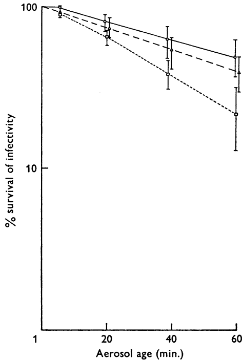
Fig. 5. The inactivation of T1 coliphage in different-sized particles in the ventilated sphere. ○, Phage in particles over 6\mu diameter; △, in particles between 6\mu and 3\mu ; □, in particles less than 3\mu . Each point represents an average of four experiments on different days at temperatures between 7^\circ and 12^\circ C. and relative humidities between 78% and 92%.
