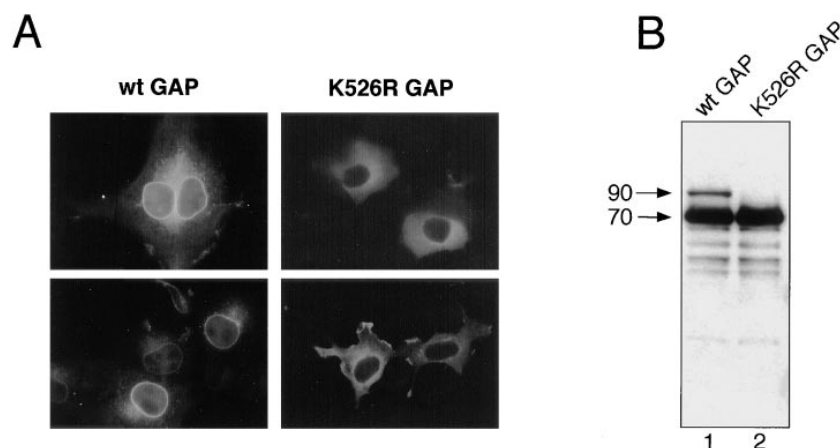
Figure 6. SUMO-1 modification of RanGAP1 at K526 is required for targeting RanGAP1 to the nuclear rim in vivo . HA-tagged wt RanGAP1 ( wt GAP ) and mutant RanGAP1 ( K526R GAP ) were transfected into Cos-7 cells and detected after 24 h. (A) Localization of transfected HA-tagged proteins by indirect immunofluorescence. Cells were fixed and probed with an α-HA monoclonal antibody. (B) Western blot analysis of transfected cells. Transfected cells were lysed by scraping into boiling SDS gel loading buffer, and analyzed by immunoblotting with α-HA monoclonal antibody.
