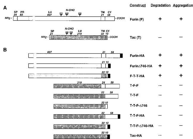
Figure 1. Schematic representation of constructs used in this study and summary of results. (A) The diagrams show the position and number of amino acid residues of the signal peptide (SP), pro-region (PR), luminal (LU), transmembrane (TM), and cytosolic (CY) domains of furin and Tac. The figure also indicates the approximate positions of sites of N-glycan addition (N-CHO) in both molecules. The gap in the furin luminal domain represents a segment that was omitted to draw the schemes to scale. (B) The diagrams represent the structures of different furin-Tac chimeras after cleavage of the signal peptide and pro-region segments. In naming the chimeras, F and T were used to designate domains derived from furin and Tac, respectively. Some of the constructs were tagged by addition of an HA epitope (YPYDVP-DYA) at the COOH terminus, as shown in the figure. In some constructs, a FLAG epitope (DYKDDDDK) was used in place of the HA epitope. The number of residues in the transmembrane and cytosolic domains of the chimeras are indicated.
