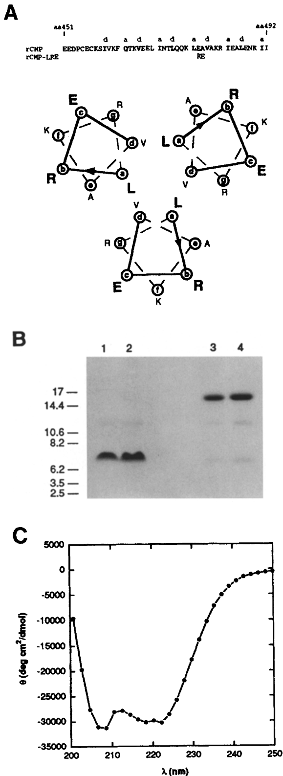
Figure 7. Characterization of the recombinant assembly domain of chicken cartilage matrix protein (rCMP). (A) Sequence of residues 451-492 of chicken CMP exons 7 and 8. The heptad repeat pattern with positions a and d occupied by nonpolar and hydrophobic amino acids is shown. Aspartate 479 and alanine 480 were mutated to arginine and glutamate, respectively, to give an LRE sequence. The position of the LRE in the triple coiled coil \alpha helix
