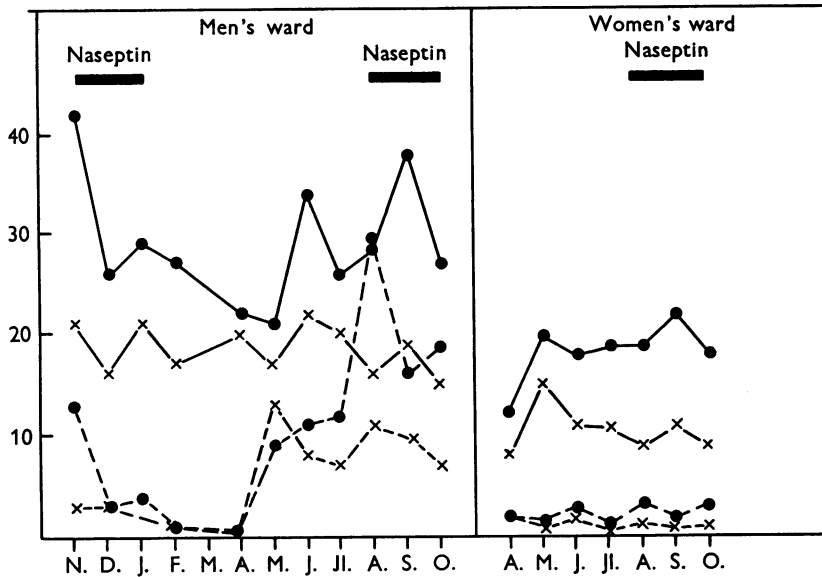
Fig. 1. Bacterial counts obtained in the men's ward, November 1960 to October 1961 and in the women's ward, April to October 1961. Monthly averages of weekly counts. ● - - - ●, Staph. aureus settling/10 sq.ft./min.; × - - - ×, Staph. aureus /10 cu.ft.; ● — ●, total bacterial count settling/sq.ft./min.; × — ×, total bacterial count/cu.ft.
