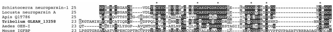
Figure 3. Sequence alignment of insect neuroparsin and related sequences. The sequences are from Schistocerca gregaria neuroparsin precursor 1 (AC38869), Locusta migratoria neuroparsin A precursor (P10776), Apis mellifera queen brain-selective protein-1 (Q1T786), Aedes aegypti ovarian ecdysteroidogenic hormone I (AAD00823), and Mus musculus insulin-like growth factor binding protein 5 protease (Mm IGFBP). Strictly conserved cysteines are marked with asterisks (*) on the top of the sequence alignment.
