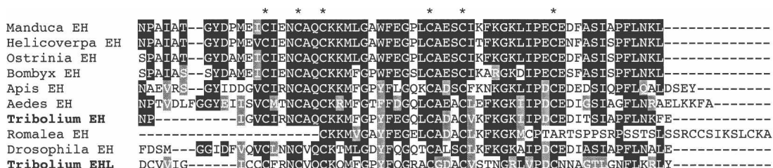
Figure 8. Sequence alignment of eclosion hormones (EH). The six conserved cysteines are marked by asterisks (*) on the top of the alignment. Sequences are from Manduca_EH (P11919), Helicoverpa_EH (AAV69026.1), Ostrinia_EH (ABG66962.1), Bombyx_EH (P25331), Apis_EH (XP_001122120.1), Aedes_EH (EAT41662.1), Romalea_EH (AAD28480.1), and Drosophila_EH (CAA51050.1).
