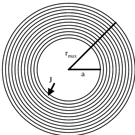
FIGURE 1 Schematical sketch of the topology used for the simulation studies. The radius of the cell is a , the maximal radius is r_{\text{max}} , and the proton flux out of the cell is J . The concentric spheres have a distance of \Delta r from each other.
