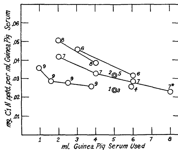
TEXT-FIG. 1. Amount of complement combining component nitrogen (C'1 N) precipitated as a function of the volume of guinea pig serum used.
