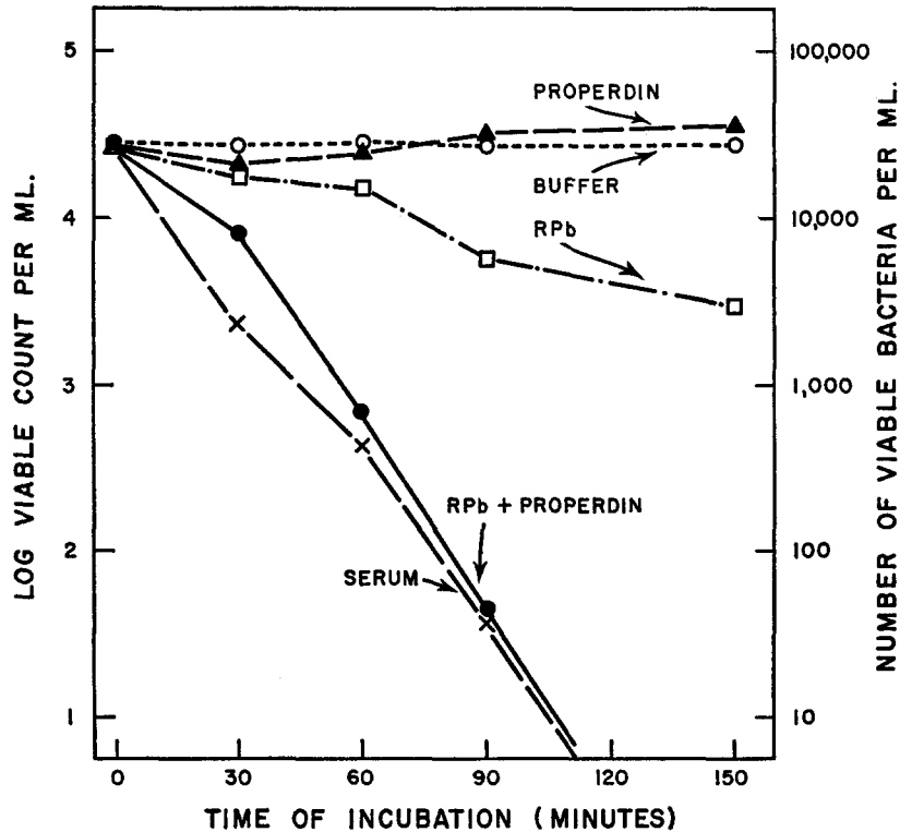
FIG. 1. The bactericidal activities of properdin, RP_b , buffer, serum, and of RP_b with added properdin on Sh. dysenteriae .
