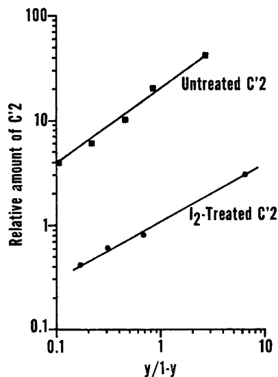
FIG. 3. Dose response for unmodified and iodine-treated C'2 plotted according to the logarithmic transformation of the von Krogh equation. y = per cent lysis; at 50% lysis y = 0.5 and y/1-y = 1 (reference 7).
