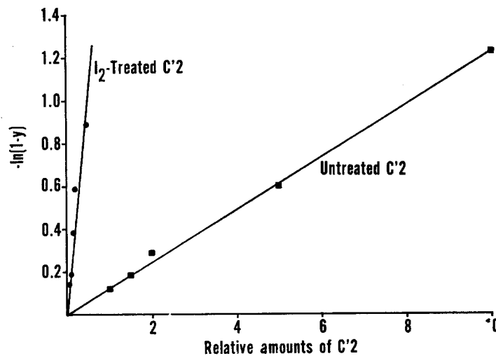
FIG. 2. Dose response for unmodified C'2, and iodine-treated C'2. Plotted as average number of C'2a sites per cell [-\ln(1-y)] .
