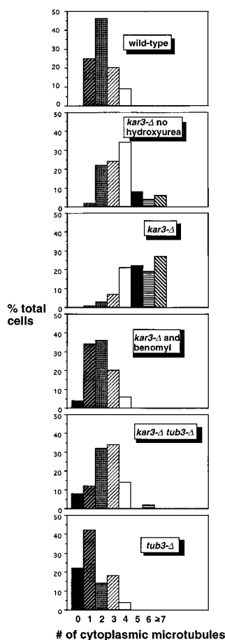
Figure 2. The increased cytoplasmic microtubule number in hydroxyurea-arrested kar3-Δ cells can be corrected by addition of benomyl or deletion of TUB3 . All samples were arrested with hydroxyurea (except as indicated) for 4 h at 26°C, fixed, and stained with anti-tubulin antibodies by indirect immunofluorescence (see Materials and Methods). Cells were examined by epifluorescence microscopy, and the approximate number of cytoplasmic microtubules was determined. Cytoplasmic microtubules were defined as those that were too long to be nuclear and/or that clearly pointed away from the nuclear envelope. Loss of Kar3p resulted in an increase in cytoplasmic microtubules, especially in the hydroxyurea-arrested culture. This defect could be mostly corrected by addition of 10 \mu\text{g/ml} benomyl to the culture medium or by deletion of the TUB3 genomic locus. tub3-Δ single mutants had fewer cytoplasmic microtubules than wild-type cells, while the
