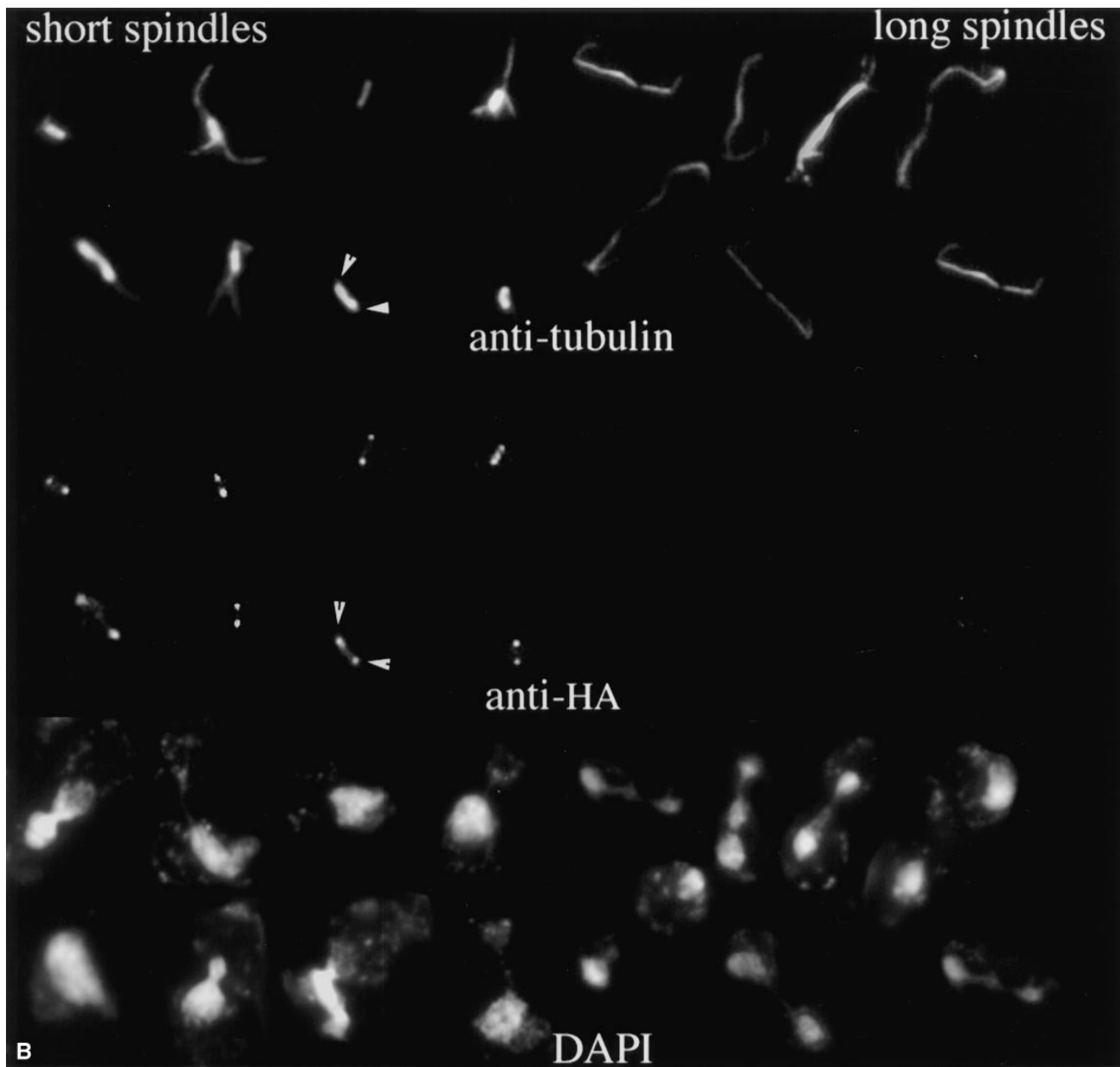
Figure 8. Immunolocalization of HA-tagged Kar3p to the spindle poles. A triple HA epitope tag was inserted near the 3' end of the KAR3 coding sequence (see Materials and Methods) and transformed into a kar3-Δ strain. (A; 1) Immunoblot with anti-HA antibodies. kar3-Δ cells with the HA-tagged KAR3 (pGD15) or with vector alone (Ycp50) were grown in selective medium. Lysed cells were run on an SDS-PAGE gel, blotted to membrane, and probed with anti-HA antibodies (see Materials and Methods). Ponceau S-stained markers from the same gel are also shown. The predicted size of Kar3p is 84 kD. Similar results were seen in multiple experiments. (2) The colony size of kar3 mutants with vector alone (Ycp50) was observed to be smaller and more varied in size than strains with KAR3 on a plasmid (pMR798). When HA-tagged KAR3 (pGD15) was transformed into kar3-Δ mutants the plasmid allowed normal colony size. Cells were grown in selective -ura medium overnight, streaked onto the same YEPD plates, and grown at 30°C for 3 d. Different kar3-Δ strains gave similar results. (3) Growth curves of kar3 mutants. kar3-Δ cells were observed to double at similar rates with plasmids containing KAR3 (▲) or HA-tagged kar3 (■), while those containing vector alone (●) divided more slowly. This test was repeated twice with similar results. (B) Cells grown to log phase were fixed briefly with formaldehyde and subjected to triple staining with antibodies to HA and tubulin and with DAPI. As shown, most of the HA-tagged Kar3p was observed to be associated with the spindle poles. The spindle pole bodies in a sample spindle are marked with arrowheads. Some intrapolar staining could be seen. Staining of intermediate length spindles varied (not shown), but long spindles from anaphase cells were invariably negative. Images shown are a composite of cells from the same sample.
