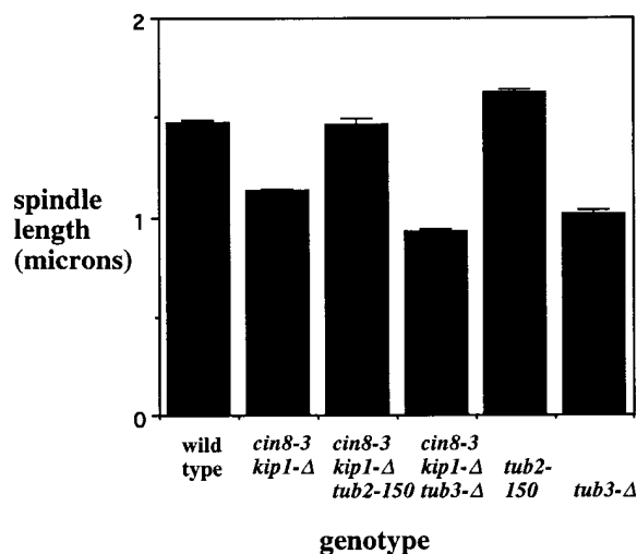
Figure 6. The short spindle phenotype from cin8 kip1 mutations is sensitive to tubulin mutations. Cells with the indicated genotypes were arrested with hydroxyurea at 26°C (a permissive temperature for growth of these strains), fixed, stained with anti-tubulin antibody, and the length of the spindles measured (see Materials and Methods). Mutational inhibition of the Cin8p and Kip1p motors produced a decrease in spindle length. This defect could be corrected by the tub2-150 mutation and was worsened by the tub3-Δ mutation. The numbers given represent the combined averages for two separate strains containing the indicated allele(s). Complete data for the individual strains are given in Table I. Each value represents at least 200 spindles counted during two to four separate experiments.
