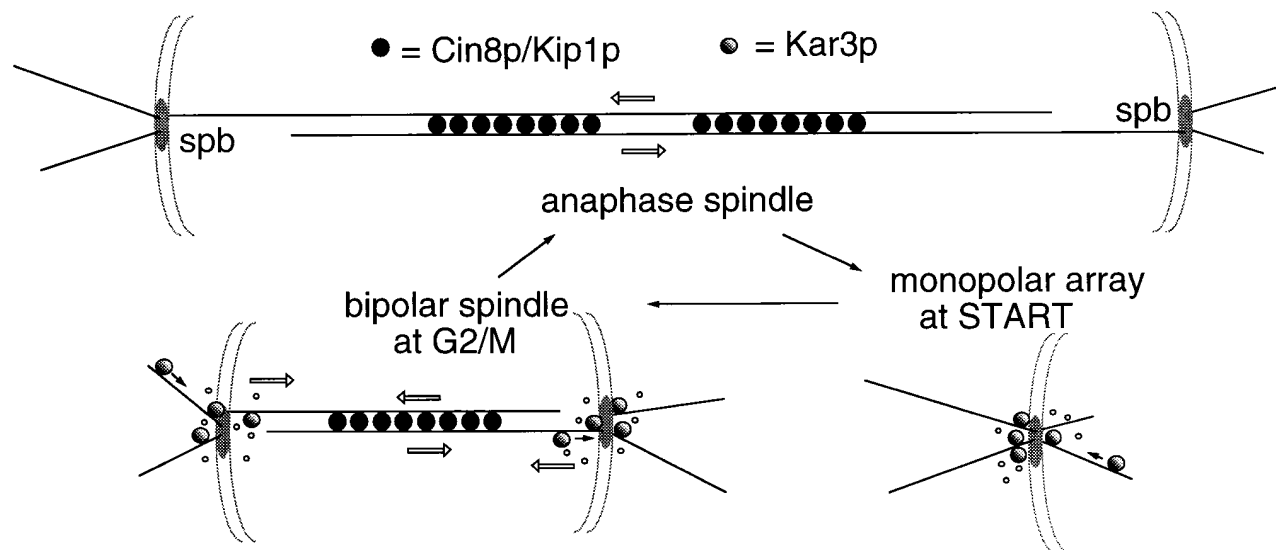
Figure 9. Model for Kar3p function in microtubule arrays. The Kar3p motor (shown as shaded circles) is proposed to function predominantly at spindle poles to stimulate microtubule turnover. At START of the cell cycle, the activity of Kar3p is required to limit microtubule number and length at the single spindle pole body ( spb ). During spindle assembly, the now duplicated spindle poles become linked by microtubule crosslinking and chromosome attachment (latter not shown). Depolymerization of the microtubules linking the spindle poles would now have the effect of pulling the poles together. Cin8p and Kip1p (dark circles) apparently function to counter this inwardly directed force, most likely by crosslinking and sliding the nuclear microtubules, using the microtubules to push out on the spindle poles (Hoyt et al., 1992) though other mechanisms are also possible. The bipolar spindle now has two types of forces acting in opposition on the spindle poles, represented by open arrows. Once anaphase begins, the antagonistic relationship between Cin8p and Kar3p changes. Kar3p-driven spindle collapse no longer occurs in cin8 kip1 mutants (Saunders et al., 1992); Kar3p is no longer found at the spindle poles, and there is a net polymerization of the spindle microtubules (and to a lesser extent the cytoplasmic microtubules) resulting in a great increase in spindle length. Thus the outwardly directed force of Cin8p and Kip1p are retained, but the inward pull of Kar3p is lost. It is proposed that this transition is a major contributor to the onset of anaphase B and can occur in the absence of chromosomes (Zhang and Nicklas, 1996). Spindle pole bodies are shown as discs embedded in a nuclear envelope, small open circles represent microtubule depolymerization, and dark arrows the presumed direction of Kar3p movement.
