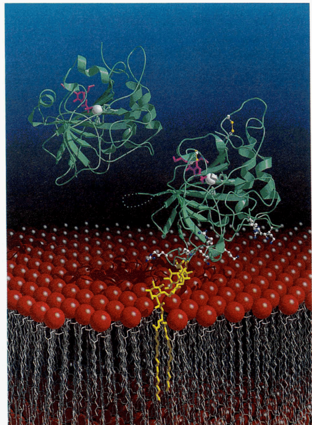
Fig. 8. CAII–brinzolamide and CAIV–brinzolamide complexes (upper left and lower right, respectively). Brinzolamide is magenta; the CAIV–membrane interaction is represented schematically, where the GPI anchor (yellow) attached to the C-terminus of the enzyme is inserted into the phospholipid bilayer. Basic residues flanking the GPI anchor stabilize the CAIV orientation by interacting with negatively charged phosphates (red). Figure prepared with MOLSCRIPT (Kraulis, 1991) and Raster 3D (Bacon & Anderson, 1988; Merritt & Murphy, 1994).
