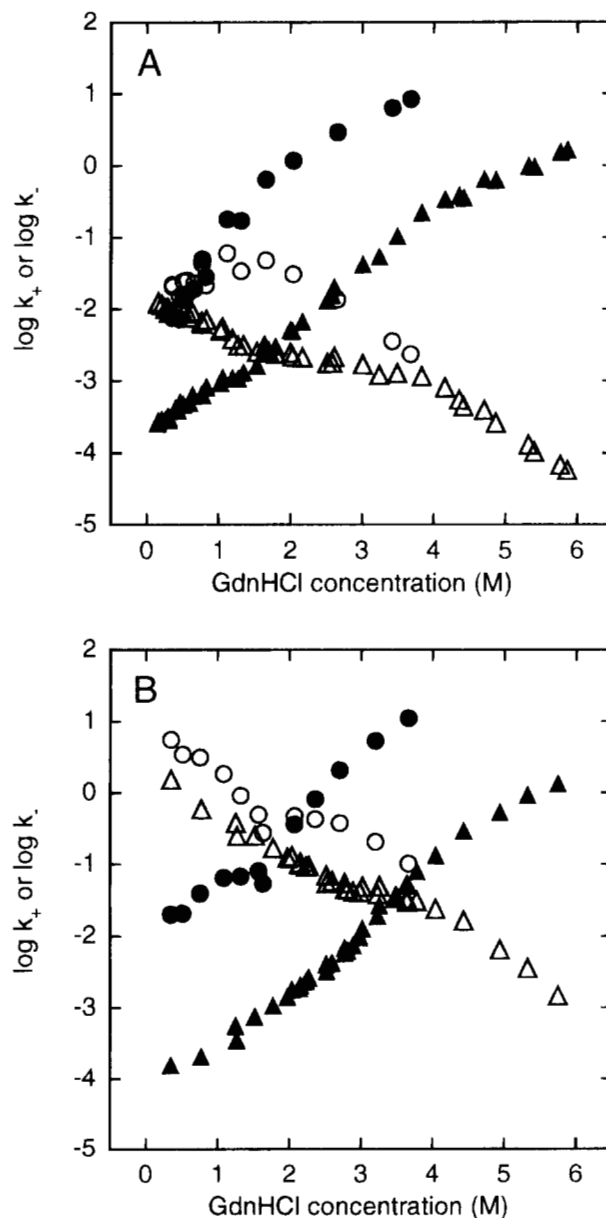
Fig. 2. GdnHCl concentration dependence of the folding ( k_+ ) and unfolding ( k_- ) rates of 2CM-3SS-BLA (circles) and intact BLA (triangles) in the absence (A) and presence (B) of 1 mM Ca^{2+} at pH 7.0 and 4.5 °C. Both k_+ (open symbols) and k_- (closed symbols) were calculated assuming that the A state is an obligate intermediate (model 1) (see text).
