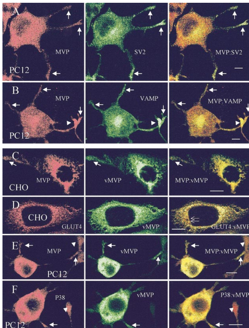
Figure 5. Localization of vault particles and vesicle markers in CHO and PC12 cells. Distribution of endogenous vaults and the synaptic vesicle marker SV2 (A) and VAMP/synaptobrevin (B) in differentiated PC12 cells is shown by double labeling in confocal images of middle sections. Arrows indicate colocalization of secretory organelles and vaults in neuritic tips. Arrowheads indicate immunostained neuritic tip of adjacent cell. An identical distribution of endogenous and recombinant MVP (vMVP) is observed in CHO (C) and differentiated PC12 (E) cells. Note, that antivault antibody (MVP) recognizes both endogenous and recombinant MVP, whereas anti-VSVG mAb only detects vMVP (C and E). Arrows indicate targeting of endogenous and recombinant MVP to cell extensions. Arrowheads indicate processes of neighboring cells revealing no or low expression of vMVP. (D) Localization of vMVP as compared to GLUT4-containing organelles is shown. Thin arrows indicate the differential distribution of GLUT4 and MVP in the perinuclear region of CHO cells. (F) Colocalization of the synaptic vesicle marker P38/synaptophysin and vMVP in neuritic extensions of differentiated PC12 cells (arrows). Arrowheads show the nontransfected cells. Bars, 10 \mu m.
