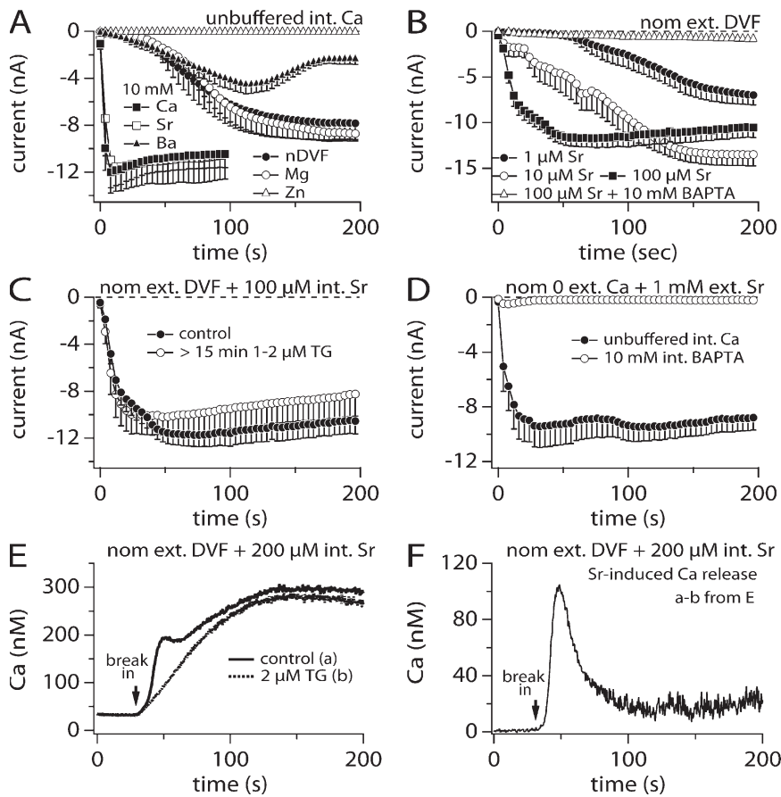
Figure 7. Substitution of \text{Ca}^{2+} with other divalent ions. (A) Average inward TRPM2 currents acquired in the presence of various individual extracellular divalent cations (10 mM) and plotted versus time. Currents were evoked by supplementing the unbuffered intracellular \text{K}^+ -based saline with 1 mM ADPR. Shown are data for nominally divalent-free conditions (closed circles, n = 7 ), 10 mM \text{Mg}^{2+} (open circles, n = 10 ), 10 mM \text{Zn}^{2+} (open squares, n = 9 ), 10 mM \text{Ba}^{2+} (closed triangles, n = 21 ), 10 mM \text{Ca}^{2+} (closed squares, n = 7 ), and 10 mM \text{Sr}^{2+} (open squares, n = 5 ). (B) Activation of TRPM2 inward currents in dependence of increasing intracellular \text{Sr}^{2+} concentrations at fixed 1 mM ADPR and in the absence of extracellular \text{Ca}^{2+} (nDVF, n = 4 –14). Intracellular \text{Ca}^{2+} was left unbuffered except in part of the dataset containing 100 \mu\text{M} \text{Sr}^{2+} (open triangles). Error bars indicate SEM. (C) Recruitment of TRPM2 inward currents by 1 mM ADPR and 100 \mu\text{M} \text{Sr}^{2+} in nDVF conditions (closed circles, n = 14 , same data as in B). The presence of 1–2 \mu\text{M} thapsigargin in the extracellular medium did not alter activation kinetics further (open circles, n = 8 ). (D) TRPM2 activation in extracellular 1 mM \text{Sr}^{2+} while keeping intracellular \text{Ca}^{2+} unbuffered (closed circles, n = 11 ) or at 0 by addition of BAPTA (open circles, n = 8 ). Pipette solution contained 1 mM ADPR. (E) \text{Ca}^{2+} signal evoked in TRPM2-
