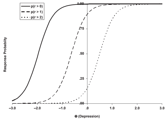
Figure 1 Boundary functions for a four-alternative item.
