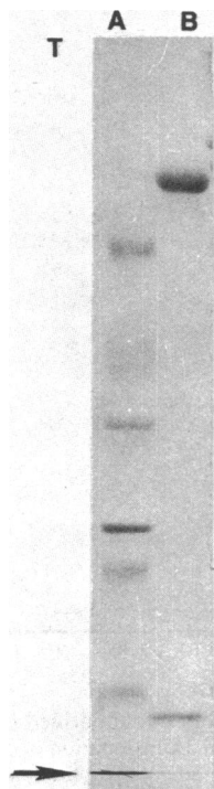
FIG. 5. Sodium dodecyl sulfate polyacrylamide gel electrophoresis of 20-fold purified CO dehydrogenase. A 10- \mu g portion of protein was applied to a 10% gel. T, Top of resolving gel; arrow, location of dye front. Lane A contains the following molecular weight standards (top to bottom): bovine serum albumin, ovalbumin, glyceraldehyde-3-phosphate dehydrogenase, carbonic anhydrase, trypsinogen, trypsin inhibitor, and alpha-lactalbumin. Lane B is the purified CO dehydrogenase, showing alpha and beta subunits (top and bottom, respectively).
