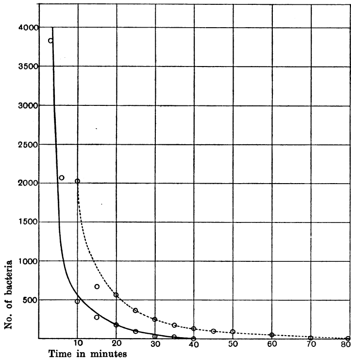
Fig. 1. Illustrating the results of Krönig and Paul's experiments. Continuous curve, disinfection of anthrax spores with 2.1 per 1000 HgCl 2 . Dotted curve, disinfection of anthrax spores with 1.1 per 1000 HgCl 2 .
