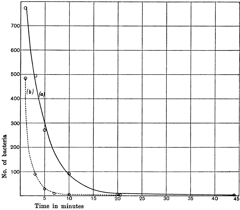
Fig. 7. ( Exp. 23. 7. 07.) Disinfection of a 24 hours' culture of B. paratyphosus with phenol, 6 per 1000, at 11° C., continuous curve: at 21° C., dotted curve (see Table VII).
