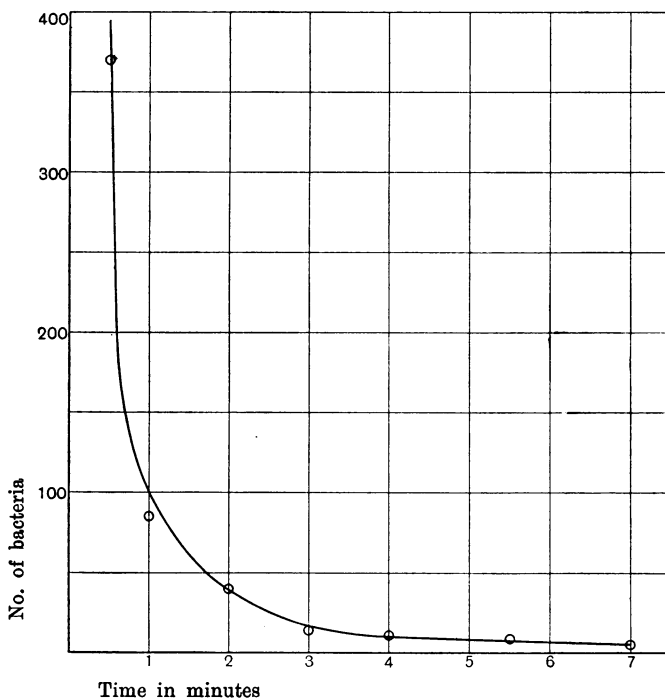
Fig. 8. (Exp. 20. 3. 07.) Disinfection of a 24 hours' culture of B. paratyphosus with disinfectant "A," 5.5 per 10,000, at 20° C. (see Table VIII).
