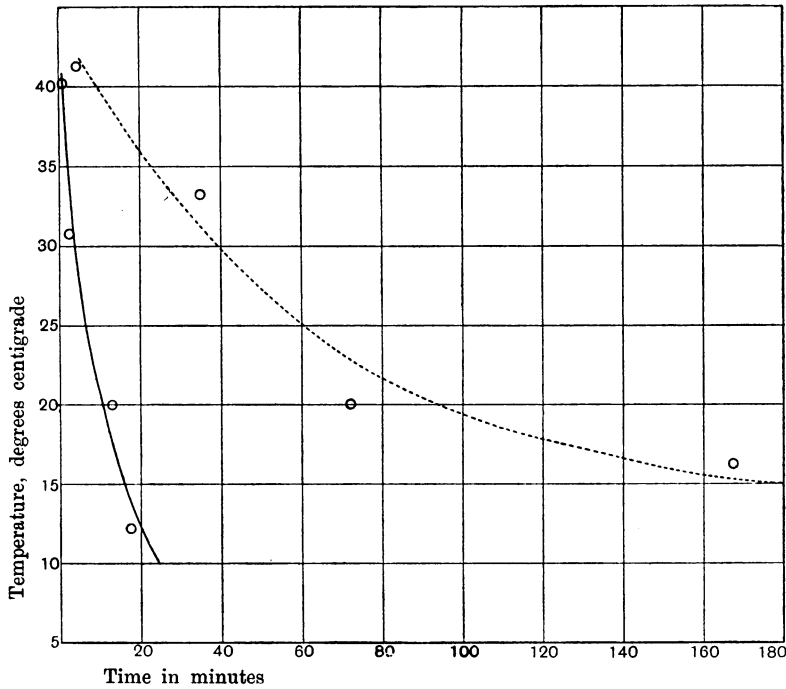
Fig. 20. Influence of temperature upon the time taken for disinfection of B. paratyphosus with silver nitrate. Continuous curve, \text{AgNO}_3 0.017 per 1000 (Table XXX, Exp. 25. 4. 07); dotted curve, \text{AgNO}_3 0.0017 per 1000 (Table XXX, Exp. 21. 6. 07).
