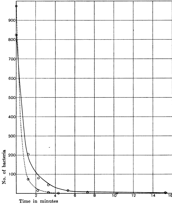
Fig. 6. (Exp. 24. 7. 07.) Disinfection of a 24 hours' culture of B. paratyphosus with phenol, 6 per 1000, at 11° C., continuous curve: at 21° C., dotted curve (see Table VI).
